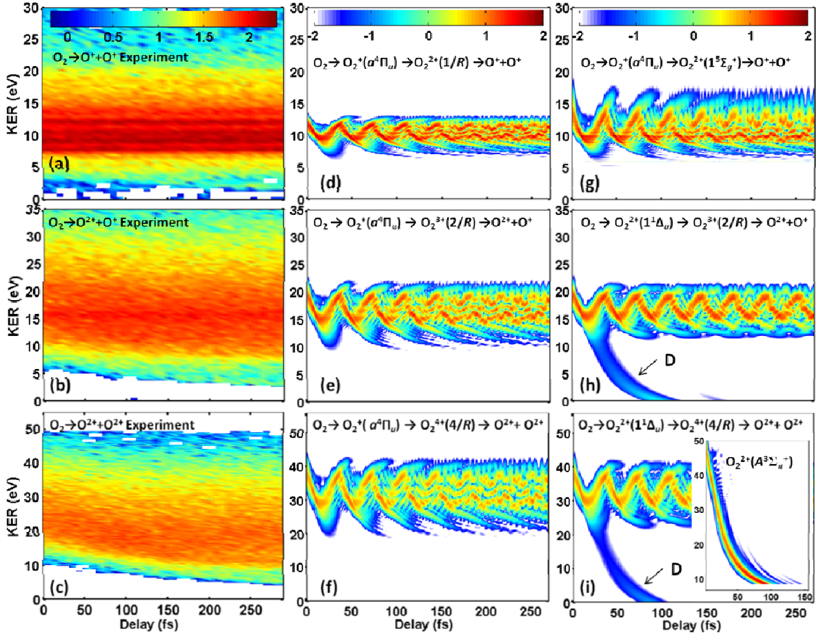
Fig. 3: (color online) (a) Measured KER spectra as a function of pump-probe delay, \tau , for the O_2 \rightarrow O^+ + O^+ break-up channel and (d, g) corresponding quantum mechanical calculations. (b) Measured KER spectra for the O_2 \rightarrow O^{2+} + O^+ channel and (e, h) corresponding quantum mechanical calculations. (c) Measured KER spectra for the O_2 \rightarrow O^{2+} + O^{2+} break-up channel and (f, i) corresponding quantum mechanical calculations (same logarithmic color/gray scales for the fragment yield within each column). The dissociation bands are marked as D (see text). The measured KER spectra are taken from Fig. 2 for positive delays and shown on a slightly different color/grey scale, as indicated. The inset in panel (i) shows the calculated KER for the dissociative intermediate state O_2^{2+}(A^3\Sigma_u^+) .
