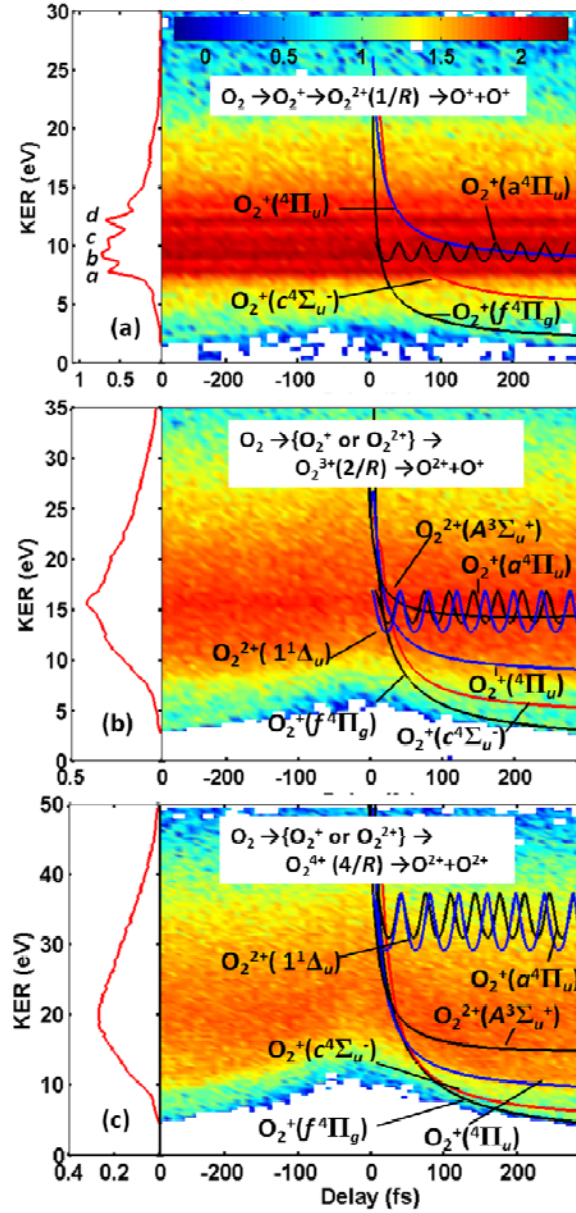
Fig. 2: (color online) Measured KER spectra as a function of the pump-probe delay, \tau , (same logarithmic color/gray scale for the fragment yield in all plots) compared with the classically calculated KER curves, K(\tau) , for different break-up channels: (a) O^+ + O^+ , (b) O^{2+} + O^+ , and (c) O^{2+} + O^{2+} . The delay-integrated KER spectra are shown on the left. The classical calculations were done using the dissociative: f^4\Pi_g , c^4\Sigma_u^- , ^4\Pi_u and bound a^4\Pi_u states of O_2^+ and the dissociative A^3\Sigma_u^+ and the bound 1^1\Delta_u states of O_2^{2+} .
