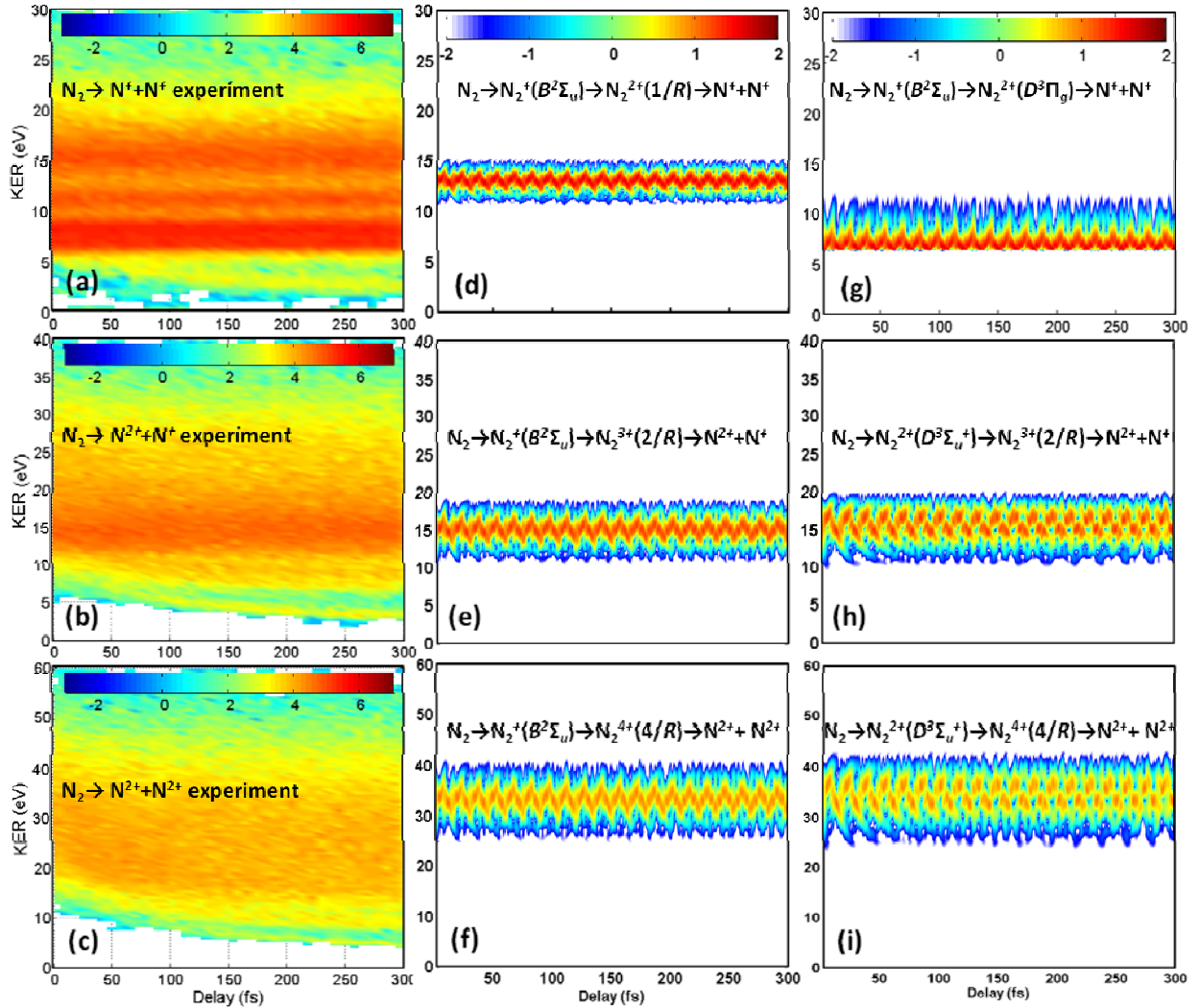
Fig. 6: (color online) (a) Measured KER spectra as a function of pump-probe delay, \tau , for the N_2 \rightarrow N^+ + N^+ break-up channel and (d, g) corresponding quantum mechanical calculations. (b) Measured KER spectra for the N_2 \rightarrow N^{2+} + N^+ channel and (e, h) corresponding quantum mechanical calculations. (c) Measured KER spectra for the N_2 \rightarrow N^{2+} + N^{2+} break-up channel and (f, i) corresponding quantum mechanical calculations (same logarithmic color/gray scales for the fragment yield within each column). The measured KER spectra are taken from Fig. 2 for positive delays and shown on a different color/grey scale, as indicated.
