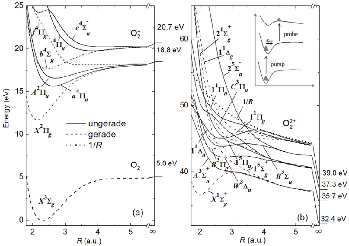
Fig. 1: Adiabatic electronic states for (a) neutral O_2 and the O_2^+ , and (b) the O_2^{++} molecular ion adapted from [26, 31, 32]. Gerade states are indicated as dashed lines and ungerade states as solid lines. The repulsive 1/R Coulomb potential, shifted to match the 39.0 eV dissociation limit, is shown as a dotted line. Dissociation limits are indicated to the right of the potential curves.
