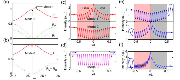
FIG. 3: (Color online) Asymmetric transmission resonances in a multi-layer heterostructure. (a) Transmittance and reflectances as a function of frequency for \text{Im}[n] \neq 0 and, (b), for \text{Im}[n] = 0 . Mode 0 is a bi-directional transmission resonance in the latter case. The structure has a constant \text{Re}[n] = 2 and consists of 50 layers with \text{Im}[n] increasing (decreasing) stepwise from 0.004 ( -0.004 ) to 0.1 ( -0.1 ) towards the center in the loss (gain) half. The frequencies are \omega L = 25.275, 25.139 in Mode 1 (wave incident from gain side) and 2 (wave incident from the loss side). Spatial profiles shown are: (c) the ATRs, (d) unitary bi-directional transmission resonance, (e) “wrong” side scattering at the ATR frequencies, and (f) “wrong” side scattering at R_R = 0 in the same structure but with larger \text{Max}[\text{Im}[n]] = 0.17 , showing a stronger asymmetry.
