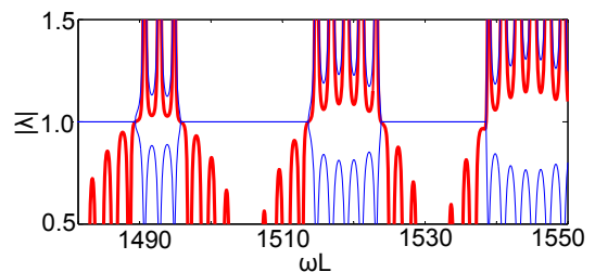
FIG. 5: (Color online) Test of the criterion (17) for \mathcal{PT} -symmetry breaking points of a three-layer heterojunction structure. The thin solid lines represent the eigenvalues of the S-matrix, which exhibit five symmetry-breaking points as the frequency \omega is tuned over the selected range. The thick solid line indicates the left hand side of Eq. (17). The heterostructure has a constant \text{Re}[n] = 3 , and the first and last layers are filled with gain and loss of \text{Im}[n] = \pm 0.005 . The width of the central passive region is 4% of the total length L .
