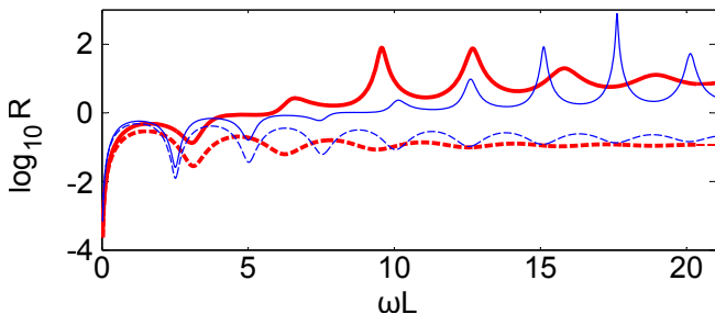
FIG. 9: (Color online) Reflectance of the gain (solid) and loss (dashed) region in the heterostructure studied in Fig. 2(a). Two values of the refractive index are considered: n = 2 \pm 0.2i (thick), n = 2.5 \pm 0.1i (thin).
