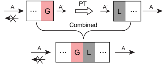
FIG. 4: (Color online) Graphical explanation of a trivial ATR arising from the transmission resonance of the left half in the right direction. \mathcal{PT} symmetry requires that it also be a resonance of the right half for left incidence (see argument in text). Depending on the particular \mathcal{PT} structure there may or may not be trivial ATRs; for example the simple heterostructure of Fig. 2(a) has no such ATRs. The ATRs of primary interest are those that arise from multiple scattering between the left and right halves of the structure.
