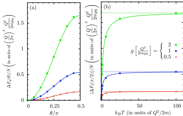
FIG. 3. (Color online) (a) The zero-point contribution to the free energy \Delta F_q as a function of \theta for three different values of g . (b) The absolute value of the (negative) thermal free energy splitting between the \theta = 0 and \theta = \pi/2 configurations |\Delta F_t(\pi/2)| as a function of temperature (solid line). This is seen to approach the quantum zero-point splitting \Delta F_q(\pi/2) at high temperatures (dashed line). In both panels the solid lines are fits to the numerically computed data points.
