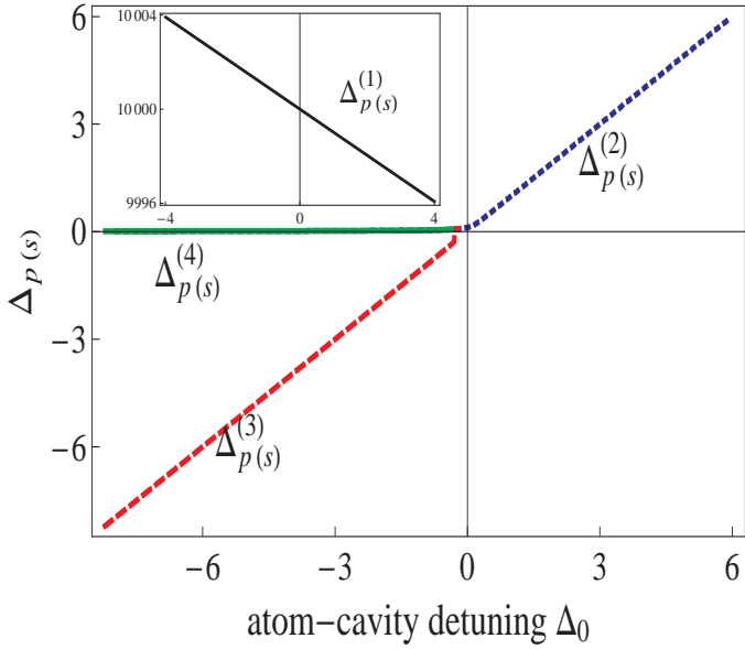
FIG. 5: (Color Online) Steady-state solutions \Delta_{p(s)}^{(i)} ( i = 1, 2, 3, 4 ) schematically shown in Fig. 2(b) versus \Delta_0 with \kappa = 10^4 . The other parameters here are the same as in Fig. 3. The inset shows the steady state solution \Delta_{p(s)}^{(1)} that corresponds to a very large displacement of the mirror. As shown in Fig. 2(b), the dotted blue, dashed red, and continuous green lines denote the solutions \Delta_{p(s)}^{(2)} , \Delta_{p(s)}^{(3)} , and \Delta_{p(s)}^{(4)} , respectively.
