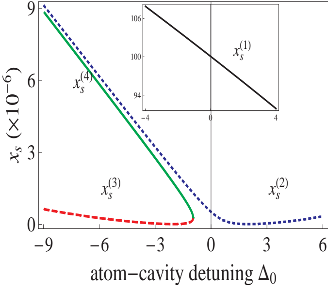
FIG. 4: (Color Online) Steady-state positions \langle x \rangle_s^{(i)} ( i = 1, 2, 3, 4 ) for the moveable mirror versus the atom-cavity detuning \Delta_0 , for the same parameters listed in Fig. 3. Here, the continuous black, dotted blue, dashed red, continuous green lines denote \langle x \rangle_s^{(1)} , \langle x \rangle_s^{(2)} , \langle x \rangle_s^{(3)} , and \langle x \rangle_s^{(4)} , when the atom-cavity detunings \Delta_{p,s} take the following steady-state values \Delta_{p,s}^{(1)} , \Delta_{p,s}^{(2)} , \Delta_{p,s}^{(3)} , and \Delta_{p,s}^{(4)} , respectively, as shown in Fig. 3.
