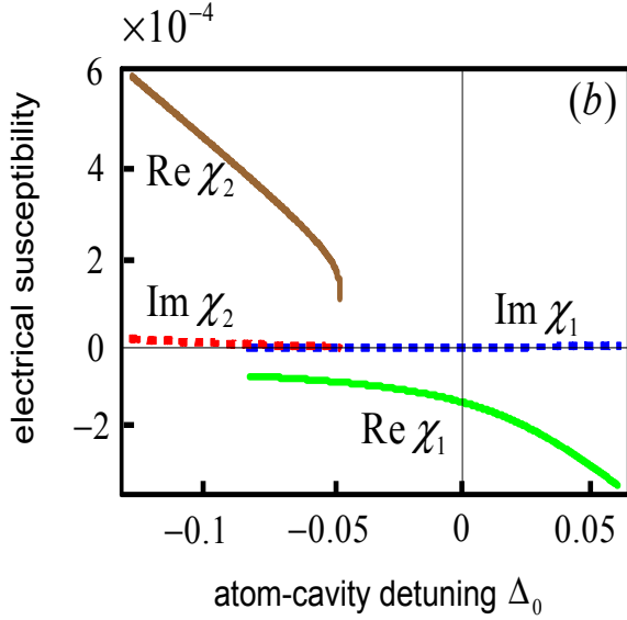
FIG. 9: (Color Online) (a) The susceptibilities \chi_1 and \chi_2 for \Delta_c = 0 and \kappa = 10^6 . (b) The magnified figure of (a) for small \Delta_0 . Here, the dotted and solid curves correspond to the imaginary and real parts, respectively. The blue and the green colors correspond to \chi_1 and the dark red and brown colors correspond to \chi_2 , respectively. It is shown in these two figures that the oscillating mirror's influence on EIT can also be observed if the detector's resolving power is high enough.
