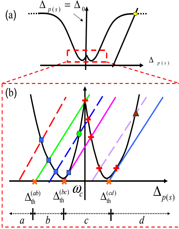
FIG. 2: (Color online) Schematic diagram for the functions of the left Y_L(\Delta_{p,s}) and the right Y_R(\Delta_{p,s}) hand sides of Eq. (28) versus \Delta_{p,s} in (a) for a large value of \Delta_0 and (b) for \Delta_0 in the region of (a) indicated by the red dashed box. In (b), the brown triangle, red crosses, green dot and blue squares denote four different steady state solutions of the self-consistent equation (28). The brown triangle (far right) denotes the solution \Delta_{p,s}^{(1)} , the four blue squares (top left) denote the solution \Delta_{p,s}^{(2)} , the red dots on the curve denotes the solution \Delta_{p,s}^{(3)} , and the green dot denotes the solution \Delta_{p,s}^{(4)} . The solution \Delta_{p,s}^{(1)} is not shown in the regions c and d. Here, \Delta_{th}^{(i)} ( i = ab, bc, cd ) denote the threshold values of \Delta_0 that separate regions with different number of solutions. Namely, \Delta_{th}^{(ab)} is the boundary point of the regions a and b, \Delta_{th}^{(bc)} is the boundary point of the regions b and c, and \Delta_{th}^{(cd)} is the boundary point of the regions c and d.
