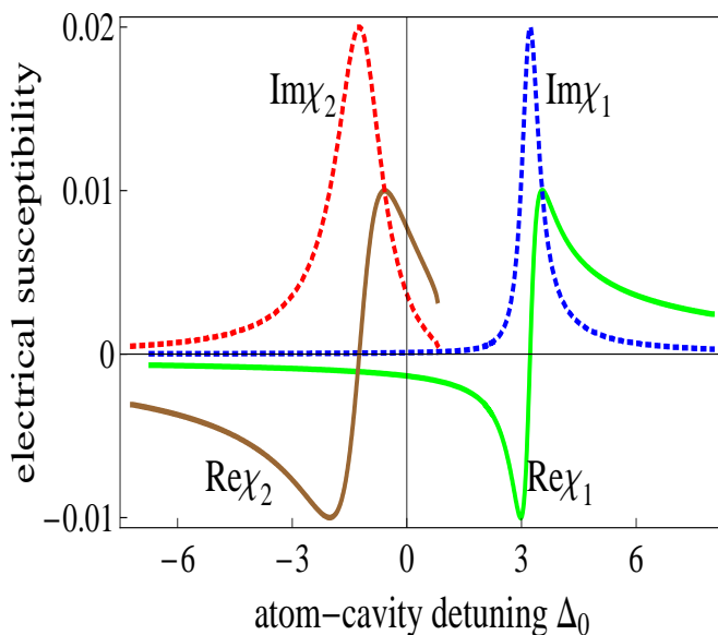
FIG. 8: (Color Online) The susceptibilities \chi_1 and \chi_2 for \Delta_c = 2 and \kappa = 10^2 . Here, the dotted and solid curves correspond to the imaginary and real parts, respectively. The blue and the green colors correspond to \chi_1 and the dark red and brown colors correspond to \chi_2 , respectively. The EIT-like region is located between the two peaks of Im\chi_1 and Im\chi_2 .
