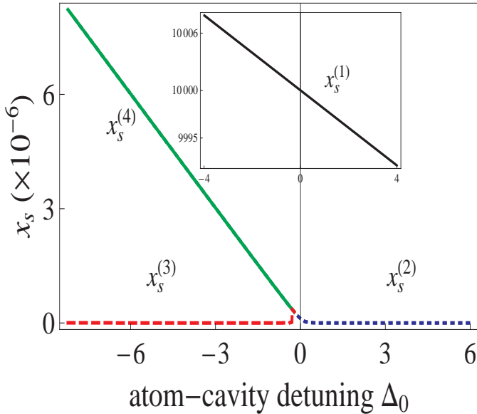
FIG. 6: (Color Online) Steady-positions \langle x_s \rangle^{(i)} ( i = 1, 2, 3, 4 ) of the moveable mirror versus the atom-cavity detuning \Delta_0 , with the same parameters as in Fig. 5. Here, the continuous black, dotted blue, dashed red, continuous green lines denote \langle x_s \rangle^{(1)} , \langle x_s \rangle^{(2)} , \langle x_s \rangle^{(3)} , and \langle x_s \rangle^{(4)} , when the atom-cavity detunings \Delta_{p(s)} (for a moving mirror) takes the following steady-state values: \Delta_{p(s)}^{(1)} , \Delta_{p(s)}^{(2)} , \Delta_{p(s)}^{(3)} , and \Delta_{p(s)}^{(4)} , respectively, as shown in Fig. 5.
