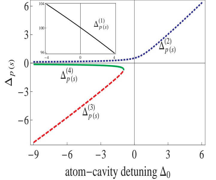
FIG. 3: (Color Online) The steady state solutions \Delta_{p,s}^{(i)} ( i = 1, 2, 3, 4 ) versus the atom-cavity detunings \Delta_0 (when the two mirrors are fixed) for given parameters, e.g., \kappa = 10^2 , \Delta_c = 0 , \omega_a = 10^6 , \gamma_0 = 10^{-6} , \gamma_2 = 10^{-4} , g = 10^2 , \Omega = 2 , and a_{in} = 10 . Hereafter, all the quantities are measured in units of \gamma_1 . Note that here eight parameters determine the system. Recall that \Delta_{p,s} is the steady-state atom-cavity detuning when one mirror is moveable. The inset shows the steady-state solution \Delta_{p,s}^{(1)} , which corresponds to a very large displacement of the mirror. As schematically shown in Fig. 2(b), the dotted blue, dashed red, and continuous green lines denote the solutions \Delta_{p,s}^{(2)} , \Delta_{p,s}^{(3)} , and \Delta_{p,s}^{(4)} , respectively. For example, the green cross in Fig. 2(b) corresponds to a single value of \Delta_0 . Here, \Delta_0 is swept, and the green cross in Fig. 2(b) becomes a continuous curve. Same for one red dot and one blue square in Fig. 2(b).
