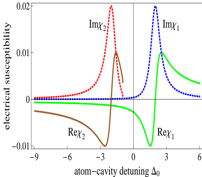
FIG. 7: (Color Online) The susceptibilities \chi_1 and \chi_2 for the detuning between the atom and the control field \Delta_c = 0 and \kappa = 10^2 . We plot only two susceptibilities because there are three stable solutions in this parameter region but two of them are quite similar. Here, the dotted and solid curves correspond to the imaginary and real parts, respectively. The blue and the green colors correspond to \chi_1 and the dark red and brown colors correspond to \chi_2 , respectively. The EIT-like region is located between the two peaks of Im\chi_1 and Im\chi_2 .
