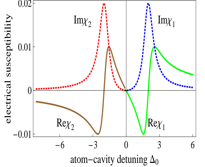
FIG. 10: (Color Online) The susceptibilities for \Delta_c = 0 and \kappa = 1.6 \times 10^{10} . Note that this value of the elastic constant \kappa is huge, corresponding to an almost fixed mirror. In this case, the Re\chi_1 and Im\chi_1 occur for mostly positive values of the atom-cavity detuning. When the spring constant becomes softer, as in Fig. 7, the Re\chi_1 and Im\chi_1 have a response that extend over a huge range of values of the atom-cavity detuning \Delta_0 , even for \Delta_c \gtrsim -6 . When \kappa tends to infinity, the susceptibility becomes the same as that in the usual EIT phenomenon. This consistency check is reassuring for our calculations. Here, the dotted and solid curves correspond to the imaginary and real parts, respectively. The blue and the green colors correspond to \chi_1 and the dark red and brown colors correspond to \chi_2 , respectively. The EIT-like region occurs near zero detuning \Delta_0 .
