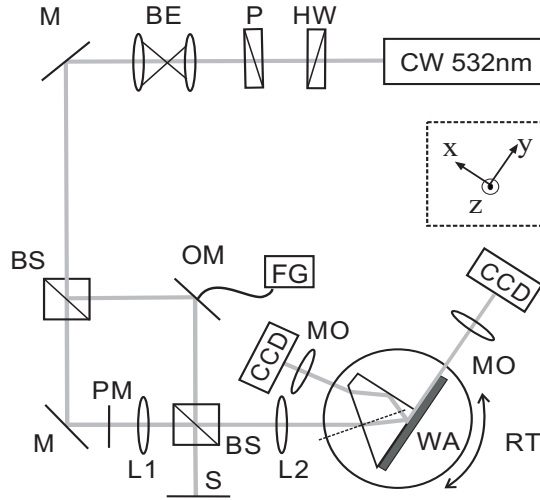
FIG. 1: Schematic experimental setup: HW, half-wave plate; P, polarizer; BE, beam expander; M's, mirrors; BS's, beam splitters; OM, oscillating mirror; FG, function generator; PM, phase mask; S, screen; L1 and L2, cylindrical lenses; MO's, microscopic objectives; CCD's, CCD cameras; PD, photodiode; WA, waveguide array.
