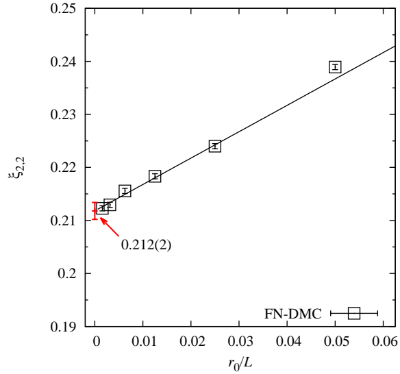
FIG. 7: (Color online) Fixed-node diffusion Monte Carlo results for \xi_{2,2} versus the r_0/L . The data is extrapolated to the limit of zero effective range.
