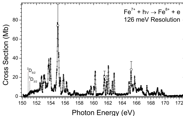
FIG. 8: Absolute cross section for photoionization of Fe^{7+} in the energy range 150 eV to 172.5 eV measured at a spectral resolution of 0.126 eV. Absolute cross-section measurements are shown by open circles with error bars, to which the energy scan data are normalized. The vertical dashed lines represent the ionization thresholds of the ^2D_{3/2} ground state and the ^2D_{5/2} metastable state.
