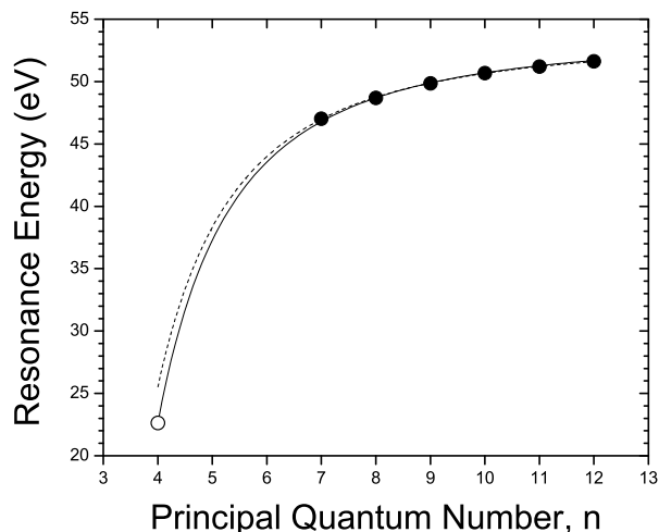
FIG. 3: Rydberg fits for the 3d^4(^1G_1) np(^2F^\circ) series from the ^2G_1 metastable state of \text{Fe}^{3+} . The solid curve was obtained by including the bound state ( n = 4 ) transition [29] (indicated by the open circle) in the fit, while the dashed curve was obtained without this bound transition.
