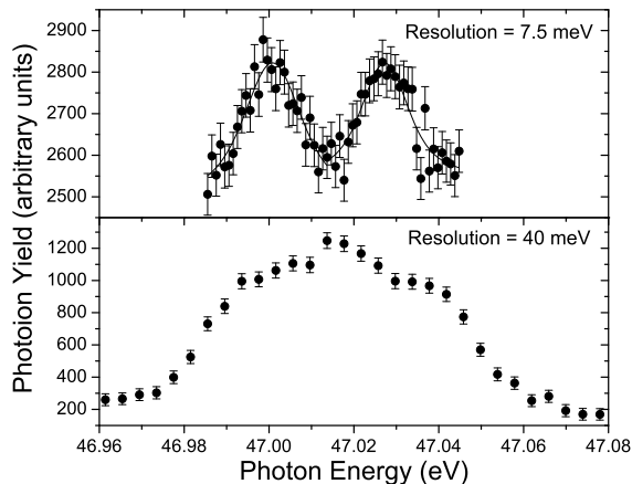
FIG. 5: Comparison of measurements of the resonance corresponding to the transition 3d^5({}^2G_1) to 3d^4 7p({}^2F^0) in \text{Fe}^{3+} at experimental energy resolutions \Delta E of 40 meV and 7.5 meV. The curve is a fit of Voigt profiles to the two resonance features.
