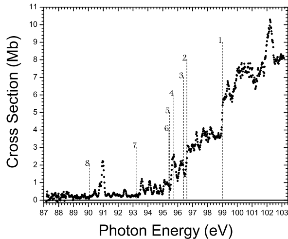
FIG. 7: Absolute cross section measurement for single photoionization of \text{Fe}^{5+} on an expanded energy scale in the range where the ionization thresholds of the eight [\text{Ar}]3\text{d}^3 terms are expected [29] and indicated by dashed vertical lines. The numbers labelling these thresholds are identified in Table III, with 1 representing the 4\text{F}_{3/2} ground state.
