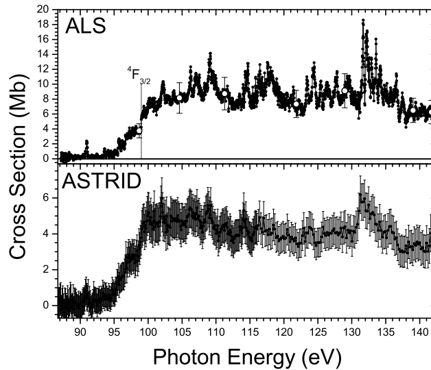
FIG. 6: Single photoionization of \text{Fe}^{5+} in the energy range 87 to 142 eV. The upper panel shows the present ALS measurements made at a fixed spectral resolution of 0.15 eV. Absolute cross-section measurements are shown by open circles with error bars, to which the energy scan data are normalized. The vertical dashed line represents the tabulated ionization threshold of the 4\text{F}_{3/2} ground state at 99.063 eV. The lower panel shows the photoionization cross section measured at ASTRID at lower spectral resolution in the same energy range [20].
