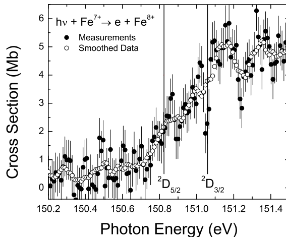
FIG. 9: Measurements of single photoionization of \text{Fe}^{7+} on an expanded energy scale in the region of the [\text{Ar}]3d\ ^2D_{3/2} ground state and ^2D_{5/2} metastable state ionization thresholds. The vertical lines indicate the tabulated values in the NIST atomic spectra database [29]. Solid circles represent the energy-scan measurements and open circles are the same measurements to which 5-point Savitsky-Golay smoothing [46] was applied to reduce the statistical fluctuations.
