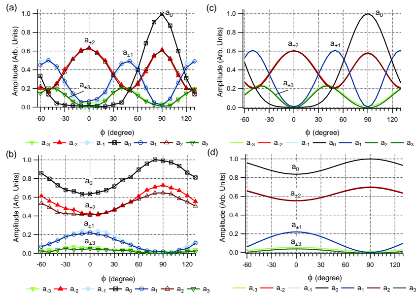
FIG. 4. (Color online) Experimental (a,b) and theoretical (c,d) dependence of the EIT resonance amplitudes on polarization angle \phi for magnetic field angles \theta = 90^\circ (top row) and \theta = 15^\circ (bottom row).
