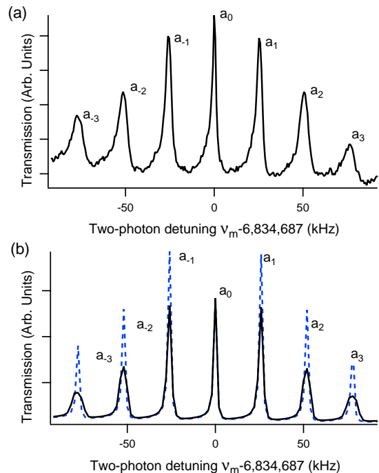
FIG. 3. ( Color online ) (a) Sample experimental EIT resonances for \theta = 90^\circ and \phi = 60^\circ with angles defined in Fig. 2. (b) Matching theoretical calculations for a perfectly homogeneous magnetic field (dashed line) and taking into account the transverse gradient from the wire (solid line).
