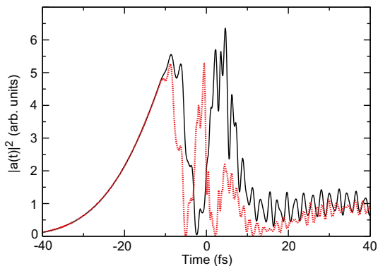
FIG. 7: (Color online). Single atom time-dependent acceleration driven by the initial XUV-IR pulse in Fig. 6. The duration of the two pulses are 61 fs and 11 fs, respectively, and the XUV intensity is 10^7 W/cm 2 . In solid black line we show the result of using an IR intensity of 1 \times 10^{12} W/cm 2 , in dashed red line the IR intensity is 3 \times 10^{12} W/cm 2 .
