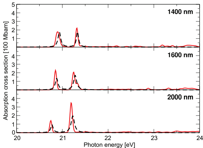
FIG. 4: (Color online) Laser-dressed XUV absorption cross section of helium for 1400, 1600, and 2000 nm laser wavelengths at a laser intensity of 10^{12} \frac{\text{W}}{\text{cm}^2} (red solid curves). The results of the simple three-level model of Fig. 5 are indicated by the dashed black curves for \Gamma_{1s^{-1}2p} = 0.1 \text{ eV} and \Gamma_{1s^{-1}2s} = 0.05 \text{ eV} .
