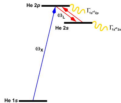
FIG. 5: (Color online) \Lambda -type three-level model for helium. The laser photon energy is \omega_L and the XUV photon energy is \omega_X . The laser-induced decay widths of the 1s^{-1}2p and 1s^{-1}2s excited states are denoted by \Gamma_{1s^{-1}2p} and \Gamma_{1s^{-1}2s} , respectively.
