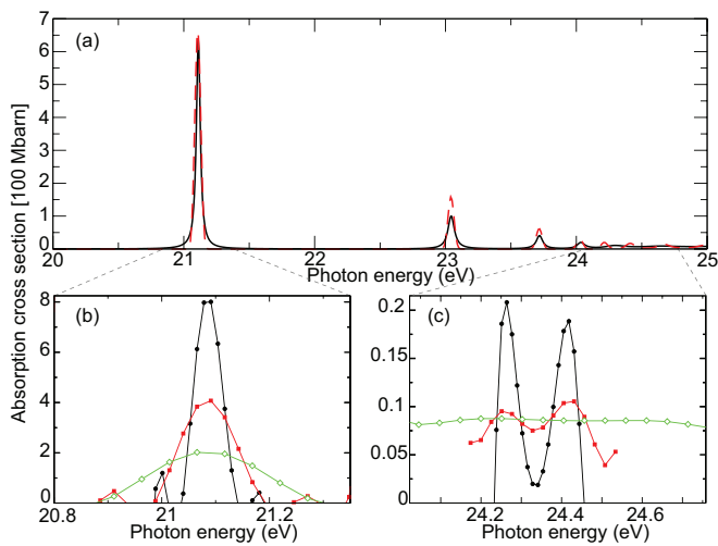
FIG. 1: (Color online) The XUV absorption cross section of a helium atom. (a) The dashed red lines were obtained with DREYD [43] the solid black lines were obtained using the TDSE-projection method. (b) and (c) show close-ups of the cross section around the 2p (b), 6p , and 7p (c) states calculated with the time-frequency method [Eq. (22)] for different XUV pulse durations. The results obtained using 30 fs, 15 fs, and 7.5 fs XUV pulses are shown in black (circles), red (squares), and green (open diamonds), respectively.
