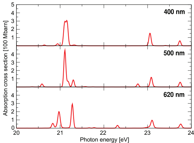
FIG. 3: (Color online) Laser-dressed XUV absorption cross section of helium for 400, 500, and 620 nm laser wavelengths at a laser intensity of 10^{12} \frac{\text{W}}{\text{cm}^2} .
