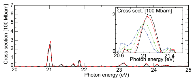
FIG. 2: (Color online) The XUV absorption cross section of a helium atom dressed by an intense 800 nm IR laser pulse with a peak intensity of 10^{12} \frac{\text{W}}{\text{cm}^2} . The dashed red lines were obtained with DREYD [43]; the cross section obtained from the TDSE-projection is plotted with dashed black lines. The inset shows the cross section calculated using Eq. (22), using an XUV pulse duration of 7.5 fs (XUV pulse duration 7.5 fs), and an 800 nm IR pulse with a duration of 15 fs and a peak intensity of 10^8 \frac{\text{W}}{\text{cm}^2} (solid black curve), 10^{11} \frac{\text{W}}{\text{cm}^2} (dashed red), 5 \times 10^{11} \frac{\text{W}}{\text{cm}^2} (dot-dashed green), or 10^{12} \frac{\text{W}}{\text{cm}^2} (dotted blue), respectively.
