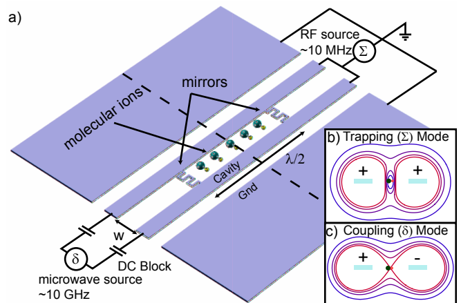
FIG. 1. (Color) a) Schematic of molecular ions trapped inside an integrated microwave resonator and split-ground ion trap. The inset shows contours of constant electric field magnitude ( |\mathcal{E}| ) in response to voltages on the two center electrodes. The two center electrodes are used both for trapping and for coupling molecules to the cavity. Electric field contours are colored from low (blue) to high (red) |\mathcal{E}| . b) The trapping ( \Sigma ) mode, when driven at \Omega_{\text{RF}} , forms a dynamically stable minimum between the two electrodes. c) The coupling ( \delta ) mode is coplanar-stripline with inductive shorts forming a half-wave ( \lambda/2 ) microwave cavity at the molecular rotation frequency ( \omega_{01} \sim 10 GHz). At the trap location, the \delta mode has a saddle point in |\mathcal{E}| , with a large electric field for coupling to the molecules' rotational dipole.
