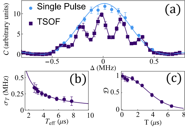
FIG. 3. (a) Contrast spectra for the single-pulse and TSOF velocimeters. \tau = 2.5 \mu\text{s} for all excitation pulses and T = 3 \mu\text{s} in the TSOF method. The solid lines are fits to Equations 1 and 3. (b) The period of the Ramsey fringe ( \sigma_T ) as a function of T_{\text{eff}} , showing a 1/T_{\text{eff}} trendline. (c) Measurements of D showing the decay of the Ramsey fringe contrast as a function of the time separation T . The solid line shows a Gaussian fit D(T) = e^{-(T/\tau_{\text{coh}})^2} , where \tau_{\text{coh}} gives \mathcal{T} \sim 5 \mu\text{K} .
