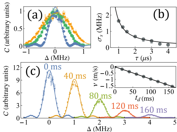
FIG. 2. (a) Lattice contrast spectra for the single-pulse velocimeter with pulse durations of 1 \mu\text{s} (yellow), 1.25 \mu\text{s} (green), and 2.5 \mu\text{s} (blue). The solid lines show fits to Equation 1 for data collected across several days from samples with slightly different c.m. velocities at t_d \approx 0 \text{ ms} . (b) Width of the contrast lineshape ( \sigma_s ) as a function of pulse duration with a 1/\tau trendline. (c) Single-pulse velocimeter contrast spectra using \tau = 2.5 \mu\text{s} , for samples interrogated at various drop times (embedded labels). The solid lines show fits to Equation 1. Inset: Velocity extracted from line-centers using Equation 2. Each velocity determination has an error of \approx 1.4 \text{ mm/s} , which is smaller than the size of the points. These data are fit to a line which gives a determination of g with an uncertainty of \approx 4.5 \times 10^{-4}g .
