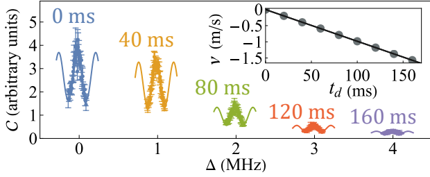
FIG. 4. Contrast spectra for the TSOF velocimeter with \tau = 2.5 \mu\text{s} and T = 3 \mu\text{s} . Signals correspond to a single Ramsey fringe collected for samples interrogated at various drop times (embedded labels). Solid lines represent fits to Equation 3. Inset: The extracted velocities as a function of drop time. Each determination has a precision of \approx 600 \mu\text{m/s} leading to a measurement of g (linear trendline) with a precision of \approx 2 \times 10^{-4} g .
