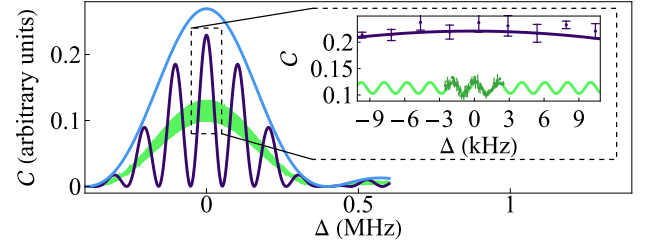
FIG. 5. Simulation of contrast spectra for a single-pulse velocimeter (light blue, \tau = 2.5 \mu\text{s} ), a short-timescale TSOF velocimeter (dark blue, \tau = 2.5 \mu\text{s} and T = 2.5 \mu\text{s} ), and a TSOF velocimeter with a large pulse separation (green, \tau = 2.5 \mu\text{s} and T = 250 \mu\text{s} ), using a sample with \mathcal{T} \approx 1 \text{ nK} . Inset: Zoomed in image where simulated data is fit to Equation 3 (solid lines), giving a velocity uncertainty of \approx 5 \mu\text{m/s} for the long-timescale TSOF velocimeter.
