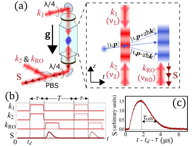
FIG. 1. (a) Schematic of the experimental setup for the matter-wave velocimeter. The excitation beams ( k_1 and k_2 ) and read-out beam ( k_{\text{RO}} ), shown by transparent red arrows, are aligned along the vertical ( z ) direction. The backscattered field ( S ) is shown by solid maroon arrows reflecting from the atomic lattice (purple). PBS: Polarizing beam splitter. \lambda/4 : Quarter waveplate. Inset: Lattice formation arising from matter-wave interference of a single ground-state |1, \mathbf{p}\rangle . Counter-propagating components of the excitation have frequencies \nu_1 and \nu_2 in the laboratory frame, both far detuned from the ground-excited state resonance. (b) Optical pulse sequence for the single-pulse (solid lines) and TSOF (dashed lines) configurations of the velocimeter at a drop time t_d , where the cold sample is released at t = 0 . (c) Time evolution of the back-scattered signal in the single-pulse velocimeter, showing the FID of the lattice with time constant \tau_{\text{coh}} .
