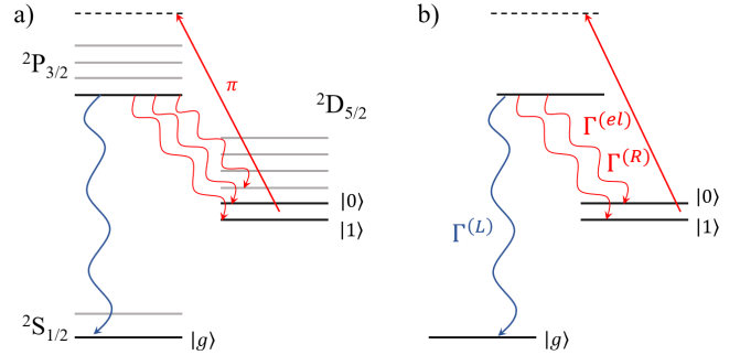
FIG. 1. (a) Partial electronic energy level diagram of ^{40}\text{Ca}^+ including metastable qubit levels |0\rangle and |1\rangle in the ^2\text{D}_{5/2} manifold. A \pi -polarized far-detuned laser beam (straight arrow) generates AC Stark shifts of the qubit levels through their interaction with the indicated ^2\text{P}_{3/2} level (black line). Off-resonant light scattering generates errors through allowed decay pathways (wavy lines). (b) Simplified level diagram used for analytic calculations with generic metastable qubits. The \Gamma^{(R)} , \Gamma^{(el)} , and \Gamma^{(L)} are rates of Raman scattering in the qubit manifold, elastic scattering, and leakage to the ground state |g\rangle , respectively.
