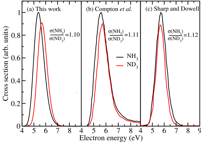
FIG. 5. Comparison of the DEA cross sections for the \text{NH}_3 and \text{ND}_3 isotopologues from the present study (panel a), and two experiments (panels b [31] and c [30]). The \text{NH}_3 and \text{ND}_3 cross sections in each panel are scaled by a factor such that the \text{NH}_3 cross section is 1 at its maximum. The ratio \sigma_{\text{NH}_3}/\sigma_{\text{ND}_3} of the peak values of the cross sections are indicated in the panels.
