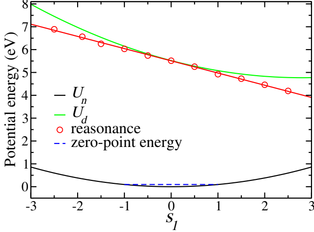
FIG. 2. Potential energy along the steepest-descent coordinate s_1 . U_n(s_1) (black solid line) is the PES of the neutral \text{NH}_3 . Resonance energies \Delta(s_1) (red line) is obtained by a linear fit using the data shown by red circles computed at discrete values of s_1 . U_d(s_1) is the anionic PES of \text{NH}_3^- obtained by adding U_d(s_1) and \Delta . Vibrational zero-point energy \frac{1}{2}\hbar\tilde{\nu}_1 is shown by the blue dashed horizontal line.
