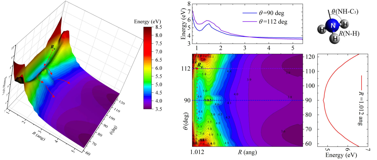
FIG. 4. PES of the 5.5 eV \text{NH}_3^- TNI state ^2A_1 as a function of the N-H nuclear distance R(\text{N-H}) and the angle \theta(\text{NH-C}_3) between the NH bond and \text{C}_3 axis. The surface is shown in the left panel. The arrows indicate the DEA flux on the surface starting from the equilibrium geometry R_e of the neutral \text{NH}_3 marked by a red dot where the incident electron is captured. The right panel shows the PES by isosurfaces. Horizontal lines representing the PES of the ^2A_1 state obtained with \theta fixed at 90 (in blue) and 112 (in violet) degrees and R(\text{N-H}) stretched, are given on the top. Red vertical lines is the PES computed
