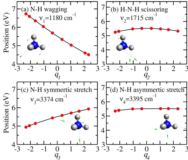
FIG. 1. Variation of the resonance energies \Delta with respect to the ground state energy of \text{NH}_3 as a function of normal coordinates: (a) q_1 of N–H wagging with \nu_1=1180 \text{ cm}^{-1} , (b) q_2 of H–N–H scissoring with \nu_2=1715 \text{ cm}^{-1} , (c) q_3 of N–H symmetric stretch with \nu_3=3374 \text{ cm}^{-1} , (d) q_4 of N–H asymmetric stretch with \nu_4=3395 \text{ cm}^{-1} . The insets display the four normal modes of \text{NH}_3 .
