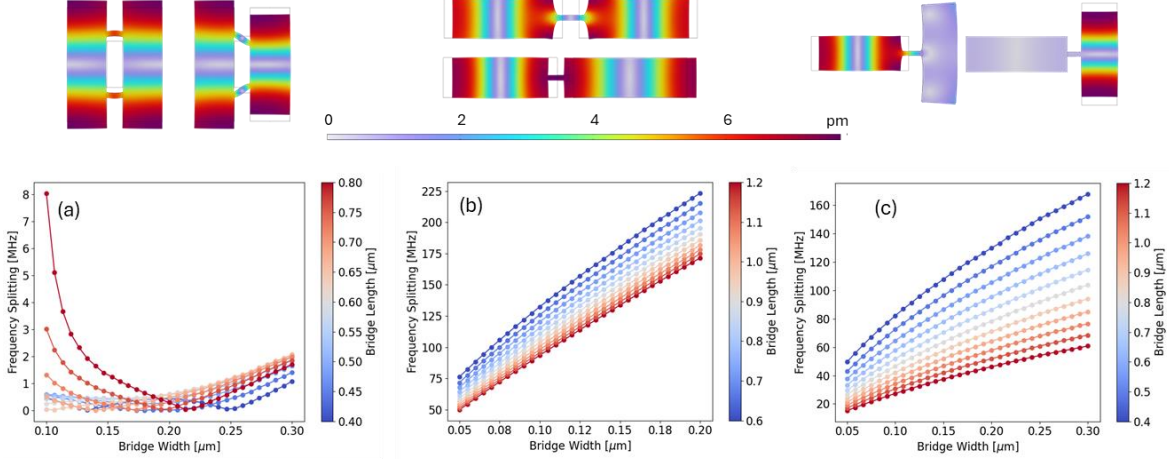
Fig. 2 (color online) Normal mode splitting of two coupled LWRs as a function of the bridge length and width. The dimensions of the LWRs are 4.25\ \mu\text{m} by 1.5\ \mu\text{m} . (a) Node-node coupling scheme, with a bridge offset fraction of 0.15. (b) Antinode-antinode coupling scheme. (c) Antinode-node coupling scheme. The top panel shows the displacement patterns of the corresponding symmetric and antisymmetric normal modes, for which the dimensions of the connecting bridges are 0.8\ \mu\text{m} by 0.2\ \mu\text{m} .
