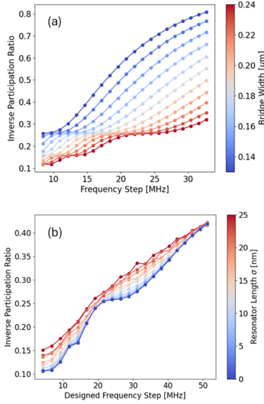
Fig. 5 (color online) (a) IPR of 1D chains of NN-coupled LWRs as a function of the frequency step and the bridge width. The bridge length is 0.6 \mu\text{m} , with an offset fraction of 0.5 . (b) The same as (a) except that the bridge dimensions are 0.8 \mu\text{m} by 0.24 \mu\text{m} and the resonator length randomly fluctuates with a Gaussian distribution and with a standard deviation of \sigma .
