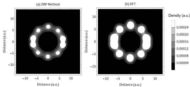
FIG. 1. The electron wave function found using the zero range potential method (a) along side the electron density (normalized to one) calculated using density functional theory (b) for one plane. The zero range potential method used \kappa as a fit parameter and \kappa = 0.85 \text{ Hartree}^{1/2} . The spots of high probability correspond to carbon nuclei. The four spots closest to the x-axis are brightest since those carbon nuclei are the closest to the plane that is being plotted.
