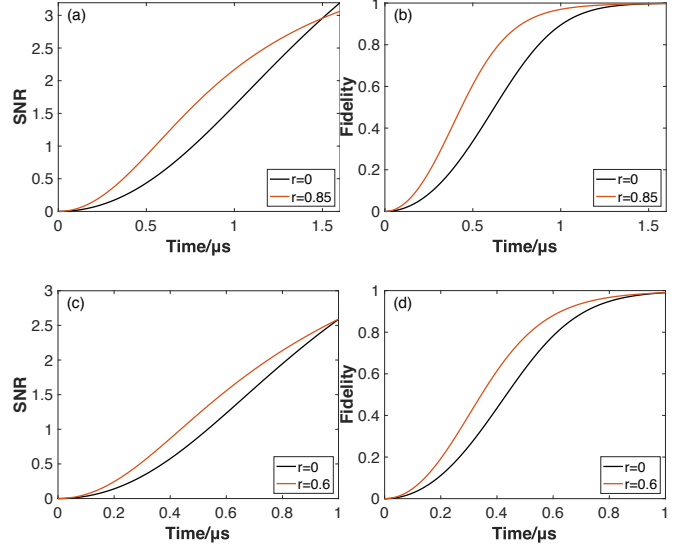
FIG. 2. SNR and readout fidelity with respect to different squeezing parameters and coupling rates. Here, \alpha = \sqrt{30} , \chi_s/2\pi \equiv 0.15 MHz, \theta_\xi = \pi , and T_1 = 3 ms [50]. The coupling rates for the panels (a), (b) and (c), (d) are \kappa = \chi_s and \kappa = 2\chi_s , respectively. The black (lower) lines represent the coherent state inputs.
