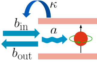
FIG. 1. Schematic of the setup for dispersive detection of spin qubits.
