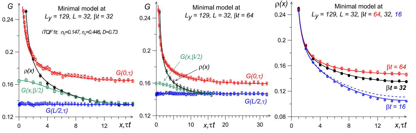
FIG. 2. Left panel: Single-particle Green's function G(x, \tau) of the minimal model (Fig. 1) along four representative space-time directions for \beta t = 32 . Solid lines are fits to the predictions of the effective iTQF theory using n_0 and D as the only fitting parameters ( n_s = 0.446 is computed from statistics of winding number fluctuations). The G(0, 0) = 0.5 point is excluded to focus on the universal low-energy behavior. Central panel: Green's function for \beta t = 64 with solid lines representing fit-free predictions of the effective iTQF theory using parameters determined for \beta t = 32 . Right panel: Density matrix \rho(x) for three different temperatures. Solid lines are theoretical predictions using parameters determined for \beta t = 32 . In numeric simulations, temperatures are known and the superfluid stiffness n_s is computed, which leaves only two fitting parameters, n_0 and D , to describe all three curves. In the experiment, where not only n_s but also temperatures may not be known, fitting the curves involves six parameters. An accurate fit thereby provides not only quantitative evidence for iTQF state and its ground state properties, but also a protocol for determining the three temperatures at which \rho(x) were measured. The dashed line for \beta t = 16 shows how the fit fails when only the state with zero phase winding is taken into account, i.e. when \Phi = 1 .
