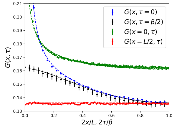
FIG. 3. Green's functions for the model Eq. (23). The dashed lines are the fits by the iTQF theory. The fit parameters have been optimized for G(x, \tau = 0) and are then reused for the other cases. The superfluid stiffness n_s = 0.5279(4) is obtained from the fluctuations in winding numbers along the x -axis, n_s = (L/\beta)\langle W_x^2 \rangle . The fit results are n_0 = 0.1481(4) and \gamma = 8.86(9) (or D \approx 1.28 ).
