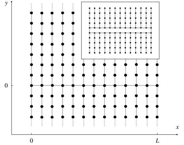
FIG. 1. Minimal iTQF model: Hard-core bosons at filling factor n = 0.5 on the square lattice, with all hopping amplitudes between sites in the x -direction suppressed, except along the single row at y = 0 . The non-zero hopping amplitudes are marked by solid lines. Inset: Image of a system of finite length with periodic boundary conditions, supporting a superflow along the central loop, which we expect to be implementable experimentally.
