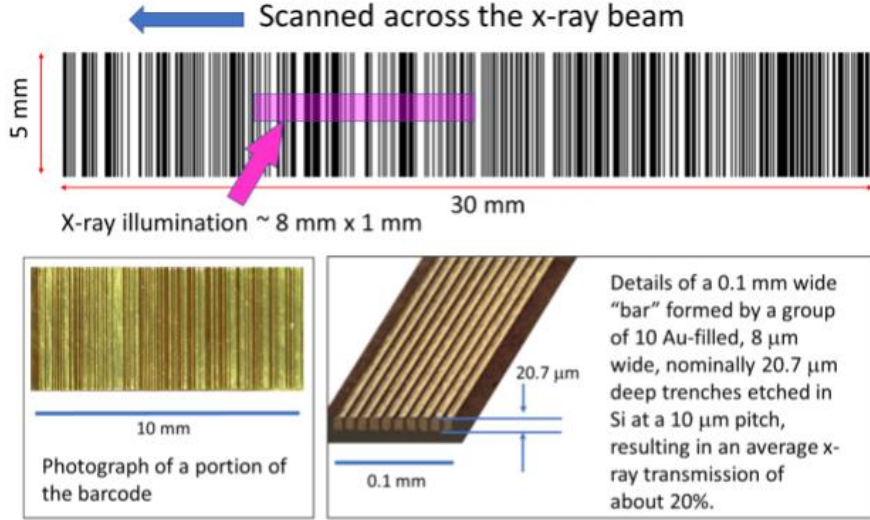
FIG. 9. The computer-designed barcode mask was fabricated by bottom-up gold filling of nominally 20.7\ \mu\text{m} deep trenches patterned and etched into the surface of a silicon wafer. The “gold” bars in the barcode pattern are actually arrays of 8\ \mu\text{m} wide Au-filled trenches and 2\ \mu\text{m} wide Si spacers that have been repeated as needed for the bar width. Illumination of the system was defined by stepping the barcode mask through a sequence of 50\ \mu\text{m} displacements parallel to the barcode, generating a total of 442 spatial patterns that were captured by a CCD camera. The same sequence of illumination patterns was repeated with the specimen in place for X-ray fluorescence data acquisition. The patterns and the corresponding XRF signals were processed offline for ghost imaging reconstruction.
