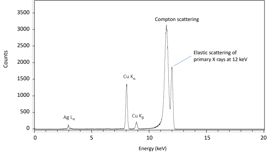
FIG. 10. An X-ray fluorescence spectrum excited by a monochromatic X-ray beam at 12 keV incident on the physical phantom made with copper wire (see photograph in FIG. 11b). The bucket signal is obtained by summing the counts under the Cu K α and Cu K β peaks. X rays that undergo elastic scattering or Compton scattering do not contribute counts to the bucket data.
