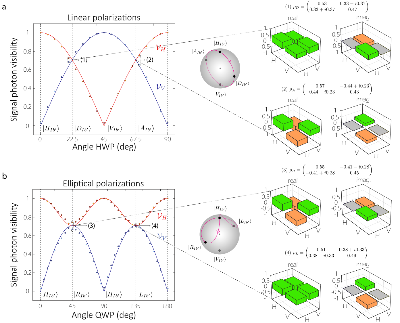
Figure 4. Experimental results for pure state tomography of photons that are never detected. Main results of visibility measurements are shown in the left panels. The red and blue colors represent the horizontal and vertical polarization, respectively. (a) The idler photon is prepared in different linear polarization states by \text{HWP}_I , see the Bloch sphere in the inset. The signal photon visibility for each linear polarization is plotted against the angle of the plate \text{HWP}_I . (b) The idler photon is prepared in different elliptical polarization states by \text{QWP}_I , starting in |H_{Ib'}\rangle . The signal photon visibility is plotted against the angle of the plate \text{QWP}_I . The calibrated experimental data points in (a) and (b) are in agreement with the theoretical predictions, which are given by the solid lines. The idler states |D_{Ib'}\rangle and |A_{Ib'}\rangle , designated by (1) and (2) in (a), and |R_{Ib'}\rangle and |L_{Ib'}\rangle , designated by (3) and (4) in (b), are all represented by the same visibilities of the signal photon. Nevertheless, these four states have different relative phases. We have included the experimental density matrices obtained for these four states in the insets (1)–(4).
