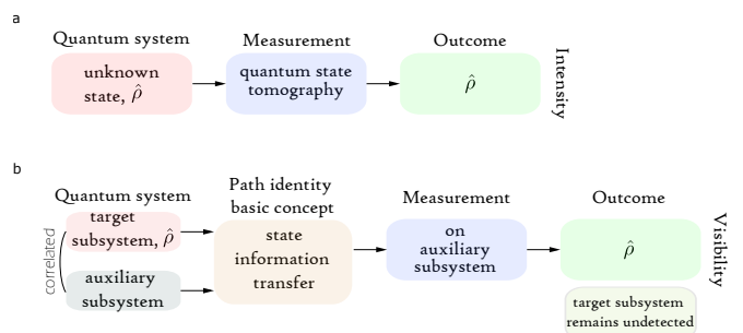
Figure 1. Quantum state tomography with detected and undetected particles. (a) Quantum state tomography retrieves the state of a quantum system by measuring an ensemble of identical particles. (b) In our scheme, the target subsystem for which we aim to obtain \hat{\rho} remains undetected. What is measured instead is an auxiliary subsystem that is quantum correlated to the target one.
