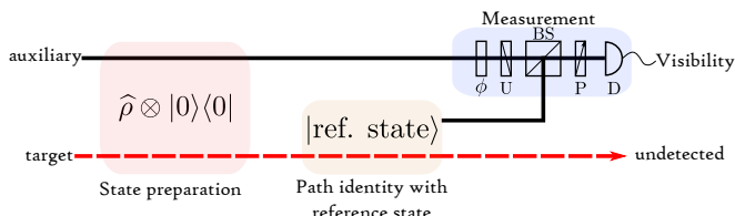
Figure 2. Path identity concept of implementation. The crucial point in our scheme is transferring the state information from the target to the auxiliary particle which is done by a path identity approach. Measurements on the auxiliary particle allow us to fully retrieve \hat{\rho} of the target particle. \phi : phase shifter, U: unitary operation, P: projector, BS: beam splitter, D: detector.
