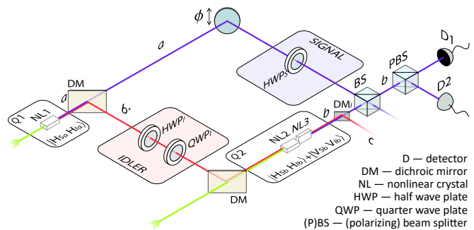
Figure 3. The experimental setup for the proposed quantum tomography method of polarization states. The pump, the idler and the signal photons are represented by the green, red and blue lines, respectively. One photon pair is created in a coherent superposition of three nonlinear crystals (NL1–NL3). Idler beams are overlapped in order to erase the which-source information, the lack of which induces coherence of the signal photon. Signal photons emitted in each crystal are superposed on a beam splitter (BS), split into H and V polarization by a polarizing beam splitter (PBS) and detected by detectors D1 and D2. The recorded intensities of the signal photon exhibit interference as the independent phase \phi is varied. Our method allows one to identify the polarization state of the idler photon emitted in crystal NL1 (source Q1) even though it is never detected. a , b , b' , and c stand for optical paths.
