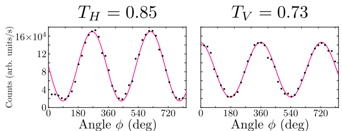
Figure 6. Experimental visibility calibration. The maximum visibility |T_H| = 0.85 \pm 0.03 is obtained from the intensity profile measured by the detector D1 when the idler photon is in the state |H_{Ib'}\rangle and the signal photon is in the state |H_{Sa}\rangle . The maximum visibility |T_V| = 0.73 \pm 0.02 is obtained for the setting |V_{Ib'}\rangle and |V_{Sa}\rangle , when the intensity profile is recorded by the detector D2. Errors are given by the standard deviation of a sinusoidal function fitted to the experimental data.
