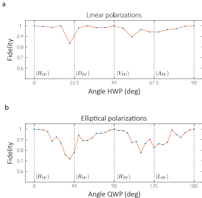
Figure 5. Fidelities of reconstructed states. (a) The fidelities for a HWP with the mean and lowest fidelities being \bar{F}_{\text{HWP}} = 0.968 \pm 0.041 and F_{\text{HWP}}^{(\min)} = 0.830 \pm 0.041 , respectively. (b) The fidelities for a QWP with the mean and lowest fidelities being \bar{F}_{\text{QWP}} = 0.916 \pm 0.074 and F_{\text{QWP}}^{(\min)} = 0.720 \pm 0.001 , respectively.
