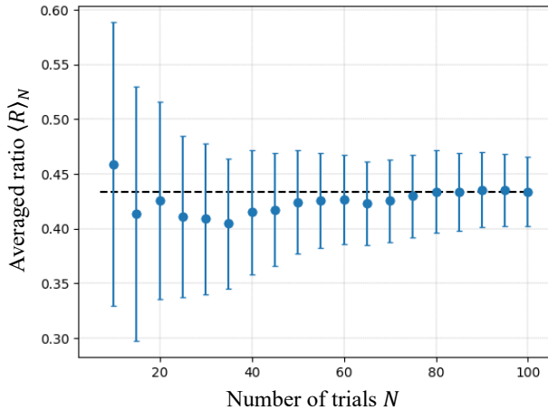
FIG. 4. Verification with IBM quantum computers: The dashed line is the exact value R_{\text{true}} = 0.433167 . The error bars represent 99% confidence interval. As we increase the number of trials N , the averaged ratios \langle R \rangle_N approach to the exact value with a clear plateau starting from N = 75 . When N = 100 , we have \langle R \rangle_{100} = 0.433706 .
