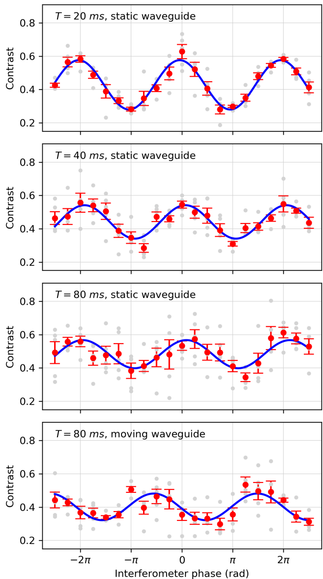
FIG. 2. Interferometer fringes for a static waveguide atom interferometer with interrogation times T = 20 , 40 and 80 ms and for a moving waveguide interferometer with T = 80 ms. Gray points represent the raw data for a single experimental run. Each red data point is an average of five repetitions for the given interferometer phase. Error bars are the standard error in those mean values.
