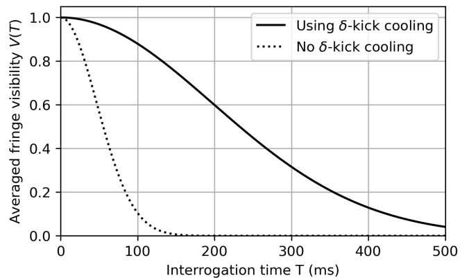
FIG. 9. The effect of phase diffusion on the fringe visibility as a function of the total interrogation time T , for N = 1000 atoms. The solid curve shows fringe visibility for an expanded \delta -kicked cooled atomic cloud, while the dashed line is calculated for the cloud before the expansion. Both calculations are based on Eq. (15) and assume constant size of the cloud during the interrogation time.
