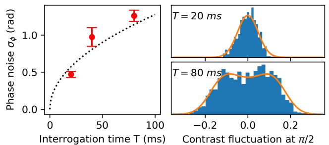
FIG. 4. Noise dependence on the interrogation time T . (left) Standard dev of the phase noise \sigma_\phi of the contrast values distribution P_i at the steep side of the fringe \phi = \pi/2 . The fit is c\sqrt{T} . (right) the histogram of the atoms fraction distribution minus the average value of the full set P_i - \bar{P} . The noise model with standard deviation \sigma_\phi determines the shape of the orange curves. Both histograms consist of about 800 samples total.
