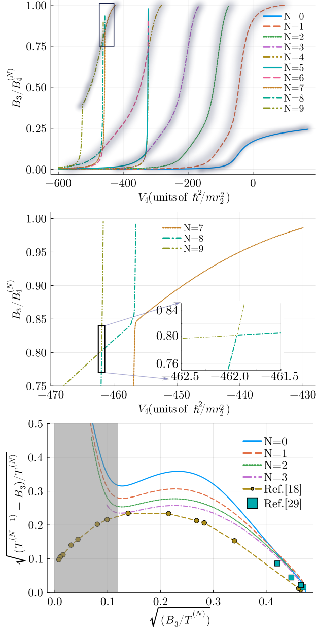
FIG. 1. Top panel: Evolution of the first ten four-bosons energy levels as a function of the strength of the four-body force V_4 . The three-boson bound-state energy is B_3 = 0.238451 \hbar^2/mr_2^2 , while the two-body system is at the unitarity limit. The four-body potential range is r_4 = r_2 . Middle panel: Zoomed-in view of the region inside the rectangle shown in the top panel. Bottom panel: The correlation cycles for the four-bosons successive universal levels. We have four cycles that have been obtained by following the universal states through the avoided crossing. The full points correspond to the universal prediction of Ref. [18], and the full squares to the separable-potential calculations of Ref. [29].
