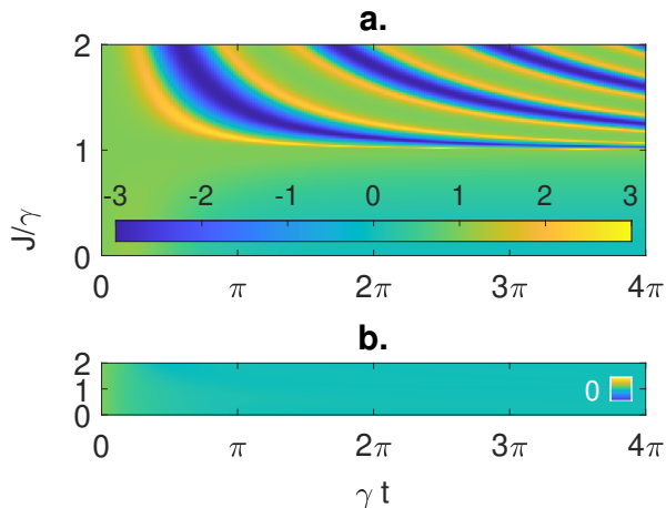
FIG. 1. LGI parameter K_3(0, t, 2t) for a fixed observable Q = \sigma_y and initial state |\psi(0)\rangle = |+_y\rangle as a function of unitless time \gamma t and inverse non-Hermiticity J/\gamma . (a) Equation of motion approach, Eq.(3), for a two-level system with Hamiltonian H(\gamma) shows K_3 varying periodically in time with a period that diverges as the system approaches the EP at J = \gamma from the Hermitian-limit side. Regions of K_3 that exceed the Lüder bound of 3/2 are clearly seen with K_3 \rightarrow 3 at the transition point. In the \mathcal{PT} -symmetry broken region J/\gamma < 1 , the non-optimized LGI parameter K_3 reaches zero at long times \gamma t \gg 1 . (b) The LGI parameter K_3 is calculated using Lindblad dynamics for a 3-level system, Eq.(5), shows a rapid decay to zero at times \gamma t \sim 1 .
