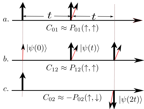
FIG. 4. Schematic of the dynamical process corresponding to the case K_3 \rightarrow 3 . In each correlation C_{01} , C_{12} , or C_{02} , only one of the four joint probabilities survives and rest are approximated to zero. Black thick arrows represent orthogonal eigenstates of the dichotomous measurement operator Q . In the \mathcal{PT} -symmetric phase, Q = \sigma_y is sufficient to maximize K_3 for all \gamma whereas in the \mathcal{PT} -broken region, the optimal Q is dependent on \gamma/J .
