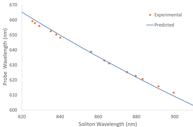
FIG. 6. Probe's output wavelength plotted as a function of soliton's wavelength (circles). Solid line is the prediction based on the dispersion data in Fig. 1.
