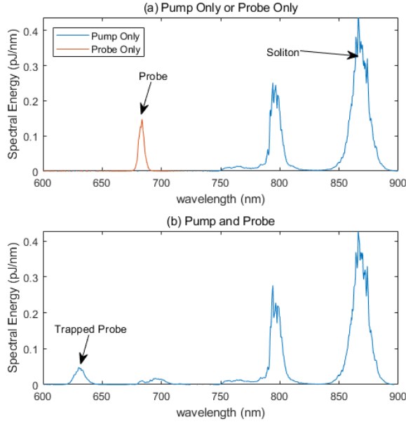
FIG. 4. Measured output spectra under different conditions. (a) Only the pump or probe pulse is sent through the PCF. (b) Both pump and probe pulses are sent through the PCF. Data are averaged over 25000 pulses.
