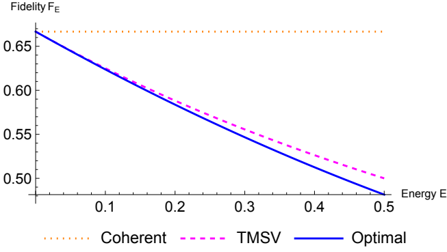
Figure 1: The graph plots the output fidelity F_E between the ideal channel and an additive-noise channel versus the input energy E , corresponding to a coherent state, a TMSV state, and the optimal state (each having input energy E ). The noise parameter for the additive-noise channel is taken as \xi = 0.5 and the states have energy E \in [0, 0.5] . The dotted (orange), dashed (magenta), and solid (blue) lines represent the output fidelity for the coherent state, the TMSV state, and the optimal state, respectively.
