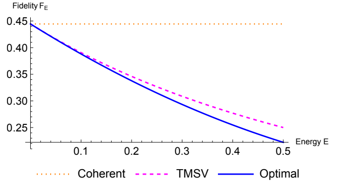
Figure 2: The graph plots the output fidelity F_E between the ideal swap channel and the tensor product of two identical additive-noise channels versus input energy E , corresponding to a tensor product of coherent states, a tensor product of TMSV states, and the optimal state (each having input energy E ). The noise parameter for the additive-noise channels is taken as \xi = 0.5 and the states have energy E \in [0, 0.5] . The dotted (orange), dashed (magenta), and solid (blue) lines represent the output fidelity for the coherent state, the TMSV state, and the optimal state, respectively.
