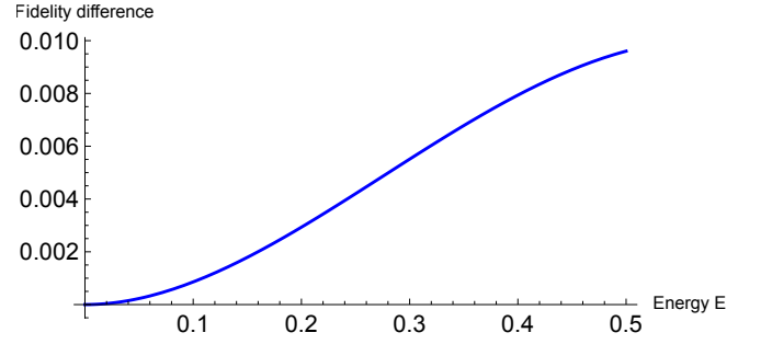
Figure 3: The graph plots the difference between the right-hand and the left-hand side of (66) versus the energy E \in [0, 0.5] for \xi = 0.5 .
