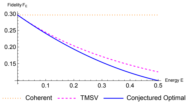
Figure 4: The graph plots the output fidelity F_E between the tensor product of three identity channels and the tensor product of three identical additive-noise channels versus the input energy E , corresponding to a tensor product of coherent states, a tensor product of TMSV states, and the conjectured optimal state (each having the input energy E ). The noise parameter for the additive-noise channels is taken as \xi = 0.5 and the states have energy E \in [0, 0.5] . The dotted (orange), dashed (magenta), and solid (blue) lines represent the output fidelity for the coherent state, the TMSV state, and the optimal state, respectively.
