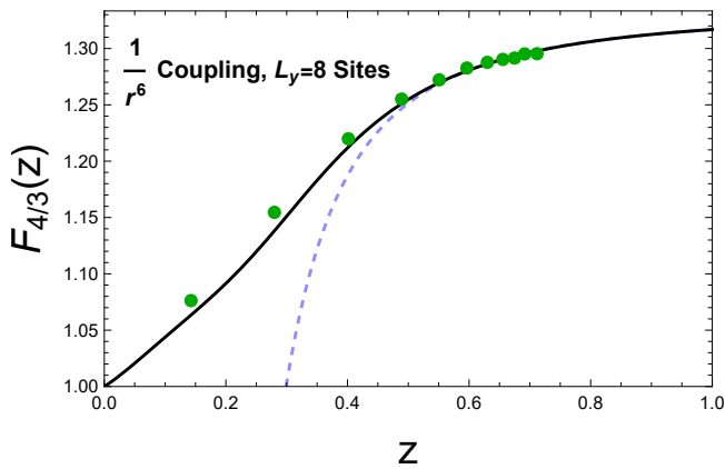
FIG. 4. F_{4/3}(z) computed by varying \frac{a_x}{a_y} for the \frac{1}{r^6} D-theory Hamiltonian for going from a lattice of size 12 \times 8 sites to 16 \times 8 sites.
