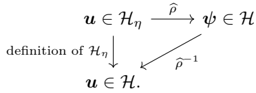
FIG. 1. The Dyson map interconnection between the various spaces.
