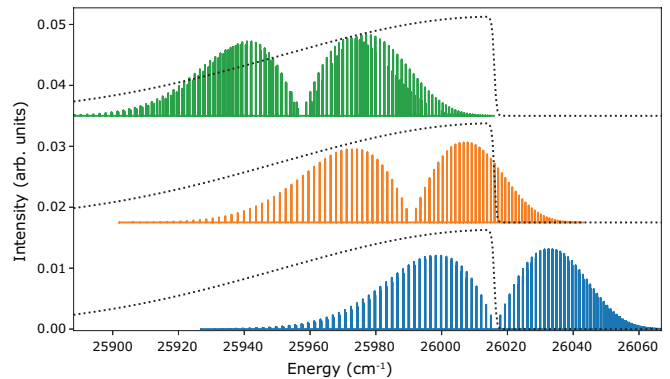
FIG. 3: Pulse shaping mask (dotted line) used to prepare the ground rovibrational state covering the B-X 0-0 (blue, bottom trace), 1-1 (orange, middle trace), and 2-2 (green, top trace) bands. The spectral separation of the P-branch ( \Delta N = -1 ) and R-branch ( \Delta N = +1 ) of \text{SiO}^+ is evident. The orange and green bands are offset in intensity for clarity.
