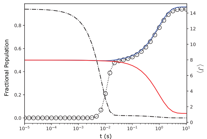
FIG. 4: Open circles - time dependence of the simulated population in the |N = 0, J = 0.5\rangle state, dashed line - fit with Eq. 8, dash-dot line - average rotational level, and the red and blue solid lines show the total population in all the odd and even total parity states respectively.
