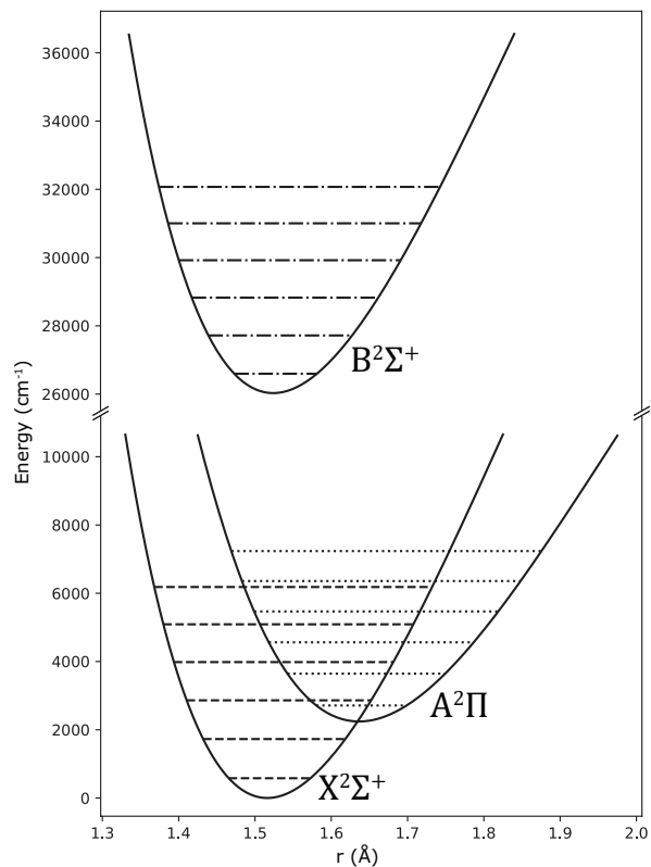
FIG. 1: The X^2\Sigma^+ (dashed for vibrational states), the A^2\Pi (dotted lines for vibrational states) and the B^2\Sigma^+ (dot-dash lines for vibrational states) are the relevant low-lying electronic states of \text{SiO}^+ for optical pumping.
