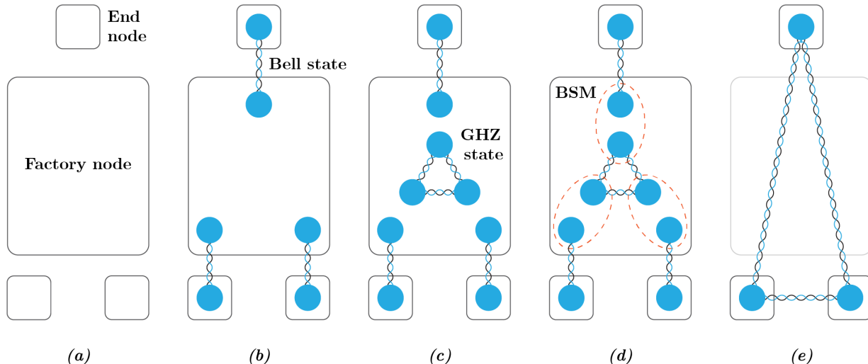
Figure 4. Illustration of GHZ-state distribution through a factory node, using Protocol 1. (a) There is one factory node, and there are N = 3 end nodes. (b) Bell states are distributed between the factory node and each of the end nodes (Step 1 of Protocol 1). (c) After all Bell states are in place, a GHZ state is created locally (Step 2 of Protocol 1). (d) BSMs are executed between qubits in Bell states and qubits in the GHZ state (Step 3 of Protocol 1). (e) If all BSMs were successful and the corresponding Pauli corrections have been applied, the end nodes share a GHZ state (Steps 4 and 5 of Protocol 1).
