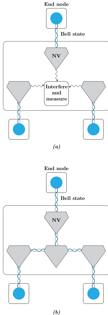
Figure 12. Implementation examples of factory nodes capable of distributing GHZ states based on NV centers in diamond. Within the factory node, N = 3 NV centers distribute and store entanglement with the end nodes. When all these NV centers are entangled, a GHZ state is distributed between them, after which each executes a BSM to teleport the GHZ state to the end nodes. (a) The GHZ state can be distributed between the NV centers by emitting entangled photons, interfering these photons, and measuring them. (b) The GHZ state can be distributed between the NV centers by first creating Bell states between all N NV centers and one additional NV center. Then, a GHZ measurement is executed at this NV center.
