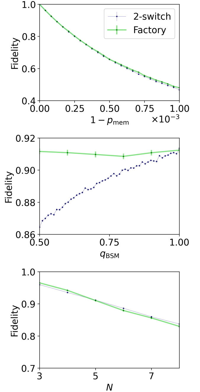
Figure 9. Sensitivity of the fidelity of Protocols 1 (“Factory”) and 2 (“2-switch”) to the memory depolarizing parameter p_{\text{mem}} , the number of end nodes N , and the BSM success probability q_{\text{BSM}} , when the only source of noise is memory decoherence ( p_{\text{link}} = p_{\text{BSM}} = p_{\text{GHZ}} = 1 ). When the parameters are not varied over, their values are p_{\text{mem}} = 1 - 10^{-4} , q_{\text{link}} = 0.01 , N = 5 and q_{\text{BSM}} = 1 . We see that when both q_{\text{link}} and 1 - p_{\text{mem}} are small, the fidelities are approximately equal for q_{\text{BSM}} = 1 and N = 5 . When q_{\text{BSM}} is decreased, this is in favor of Protocol 1. However, if N is increased, this is slightly in favor of Protocol 2. Note that the lines in the top (and to lesser degree, the bottom) figure can be hard to distinguish because of their overlap.
