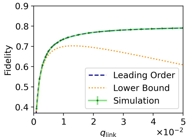
Figure 5. Comparison between simulation result and analytical expressions for the fidelity of Protocol 1. The parameters are N = 5 , q_{\text{BSM}} = 0.95 , p_{\text{BSM}} = p_{\text{link}} = 1 - 10^{-2} and p_{\text{mem}} = 1 - 10^{-4} . GHZ states are locally prepared with a fidelity of 0.9, which corresponds to p_{\text{GHZ}} \approx 0.872 . The lower bound is tight for small values of q_{\text{link}} , but not for larger values. The leading-order expression on the other hand stays accurate also for larger values of q_{\text{link}} . Each data point represents the average over 10,000 simulated executions of Protocol 1. Error bars represent the standard deviation of the mean and are smaller than the markers. Note that the lines showing the leading-order result and the simulation result can be hard to distinguish because of their overlap.
