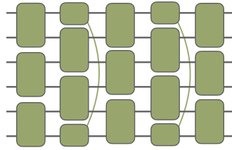
FIG. 3. A brickwork circuit as being a subject of Theorem 1. Periodic boundary conditions impose a gate (green boxes) on qubits n and 1 in each even-indexed layer.
