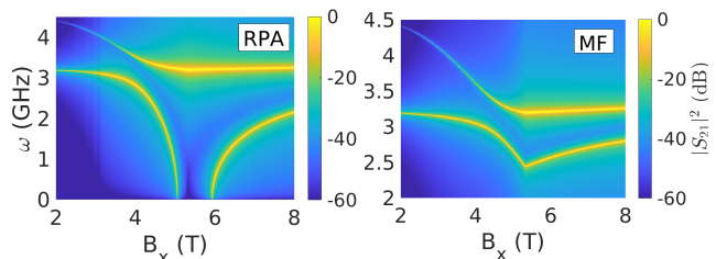
FIG. 4: Damped transmission function of LiHoF 4 in a 3.2GHz microwave resonator with a filling factor of \eta = 0.25 in the RPA (left), and in MF theory (right). We consider the zero temperature transmission of a LiHoF 4 sample with zero average demagnetization field. The damping parameters are given by \Gamma_m \propto A_m \omega_m^2 (similarly for the MF modes). The proportionality constant is chosen so that the damping parameters are roughly in line with what one expects for spin vacancies in diamond (see text). In the RPA (left), the damping is insufficient to prevent superradiance in the system due to the divergent spectral weight of the magnon soft mode. The spectral weight carried by the lowest MF mode does not diverge, and the resultant coupling strength is not strong enough to cause superradiance in the single ion resonator spectrum (right). In a system subject to decoherence, one expects to see both single ion and collective mode transmission.
