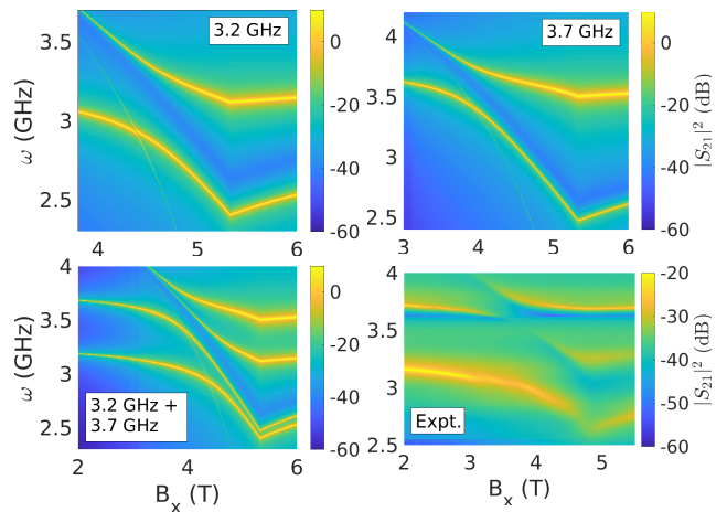
FIG. 6: Mixed single ion and collective mode transmission of LiHoF 4 in a 3.2GHz and 3.7GHz resonator at zero temperature. The filling factor is set to \eta = 0.25 , and the damping parameters are chosen to be in line with what one expects for spin vacancies in diamond. The decoherence factor is set to \gamma_{dec} = 100GHz , a value for which, although faint, the soft mode is visible in the transmission spectrum. Comparing the avoided level crossing in the 3.2GHz resonator to the 3.7GHz resonator in the upper pair of figures, we see a larger avoided level crossing at the lower frequency. This is due to the increase of the spectral weight of the magnon mode at 3.2GHz, which supersedes the reduction in coupling strength due to the lower resonator frequency. In the lower pair of figures, we sum the calculated transmission from the 3.2GHz and the 3.7GHz resonators, and compare the results to transmission through a bimodal loop gap resonator. In the experimental data, interactions between the resonator modes lead to an antiresonance near 3.6GHz and hybridization of the polariton modes not accounted for in the theoretical calculation. The lowest polariton mode in the experimental data exhibits weak avoided level crossings consistent with the presence of the collective soft mode, and Walker modes, in the material (see text for details).
