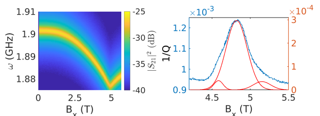
FIG. 3: Measured transmission function of LiHoF 4 in a 1.9GHz microwave resonator. The inverse quality factor of the resonator mode is shown on the right. The measured value of 1/Q (blue) has been decomposed into the sum of three Gaussian peaks (red). The central peak corresponds to absorption at the phase transition. The satellite peaks to either side of the central peak occur where the soft mode is degenerate with the resonator mode.
