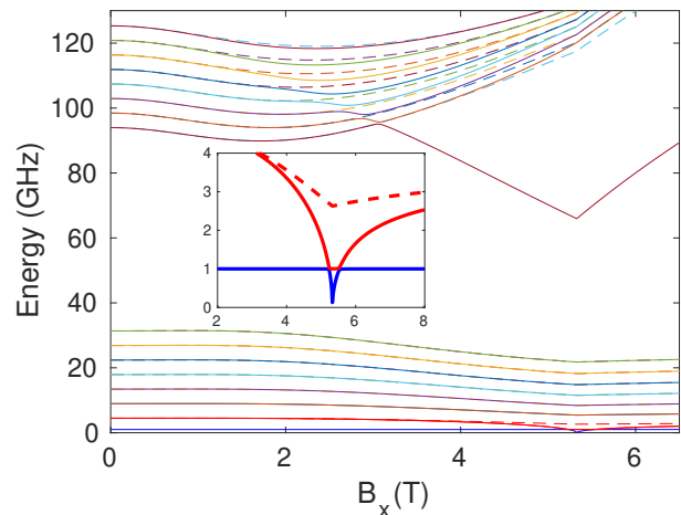
FIG. 1: Modes of \text{LiHoF}_4 , at zero temperature, in a 1GHz resonator with a filling factor of \eta = 0.01 . We assume the average demagnetization field in the sample is zero. Due to the weak coupling, the RPA modes of the resonator are much the same as the RPA modes of \text{LiHoF}_4 , with an additional mode at the resonator frequency. The MF modes of the \text{LiHoF}_4 system are shown as dashed lines for comparison. The mode showing significant softening in the upper band of energy levels has dominant spectral weight. This mode has been measured in neutron scattering experiments 39 . In the inset, we see the lowest energy electronuclear mode soften to zero at the quantum critical point. A similar figure showing the electronuclear modes of \text{LiHoF}_4 , and their spectral weights, is provided in reference 16 .
