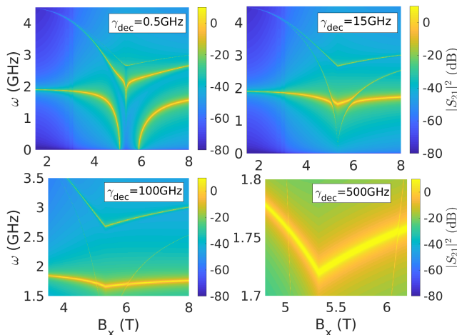
FIG. 5: Mixed single ion and collective mode transmission of a LiHoF 4 sample in a 1.9GHz resonator at zero temperature. The filling factor is set to \eta = 0.25 and we assume the average demagnetization field is zero. The damping parameters are chosen to be in line with what one might expect for spin vacancies in diamond. In the upper left figure the decoherence factor is set to \gamma_{dec} = 0.5GHz . The sharp dip in the upper polariton mode occurs where the soft mode crosses \gamma_{dec} . In the upper right figure the decoherence factor has been increased to \gamma_{dec} = 15GHz , which is sufficient to prevent superradiance. Further increasing the decoherence factor attenuates the soft mode and closes the avoided level crossing in the spectrum. In the experimental data, one expects a weak avoided level crossing to show up as a resonance in the inverse quality factor of the resonator.
