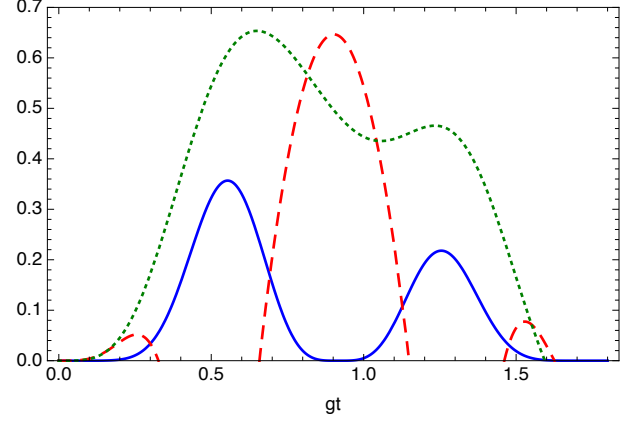
FIG. 6: Entanglement for the case N = 4 and n_0 = 3 as detected by inequalities (53) (solid line), (57) (bipartite entanglement, dashed line), and Eqs. (52) (dotted line). Note that the solid line is actually always above zero except at gt\sqrt{14} = 2n\pi , whereas the other two cross the horizontal axis with a nonzero slope. Note also the existence of a small region to the right where the dashed line detects entanglement but the dotted one does not.
