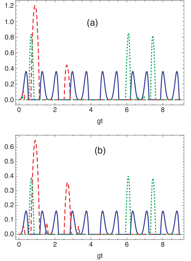
FIG. 4: Entanglement between subsystems for N = 4 atoms starting in the ground state and interacting with n_0 = 2 (solid line), 3 (dashed line) and 4 (dotted line) photons. (a) One atom in subsystem a , three in subsystem b (inequalities (48)). (b) Two atoms in each subsystem (inequalities (52)).
