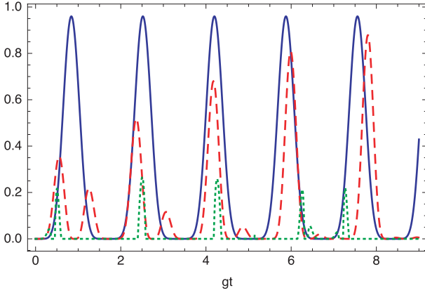
FIG. 5: Entanglement between subsystems of two atoms each, for a total N = 4 atoms starting in the ground state and interacting with n_0 = 2, 3 and 4 photons, as detected by inequalities (53).
