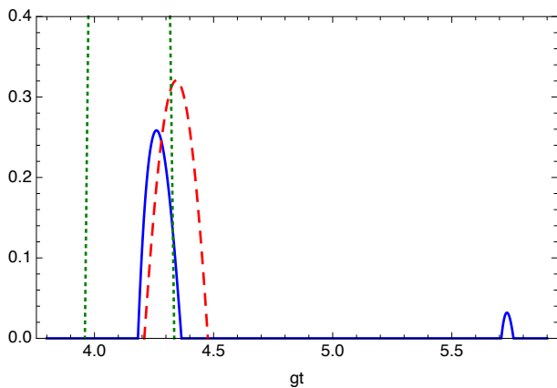
FIG. 7: Entanglement for the case N = 4 and n_0 = 4 as detected by inequalities (53) (solid line), (57) (bipartite entanglement, dashed line), and (58) (genuine tripartite entanglement, dotted line). Note that the three criteria overlap in places, but there are also times when entanglement is only detected by one of them.
