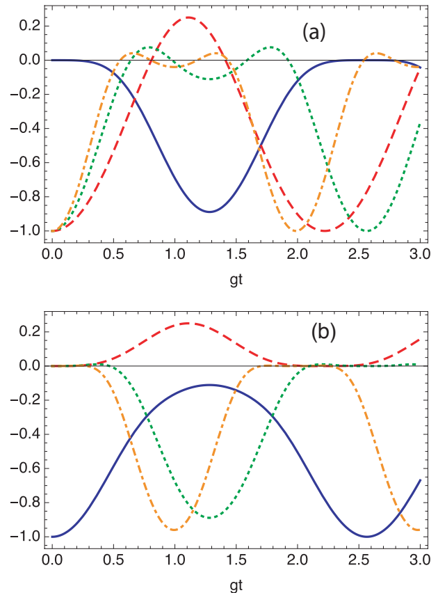
FIG. 1: (a) The difference \frac{1}{4}|c_0(t)|^4 - |c_{-1}(t)|^2 (positive values indicate an entangled state of the two atoms) for four different cases: pure spontaneous decay ( m_0 = 1, n_0 = 0 , solid line), and evolution from the ground state with n_0 = 1 (dashed line), 2 (dotted line) and 3 (dot-dashed line) photons respectively. (b) The same for \frac{1}{4}|c_0(t)|^4 - |c_1(t)|^2
