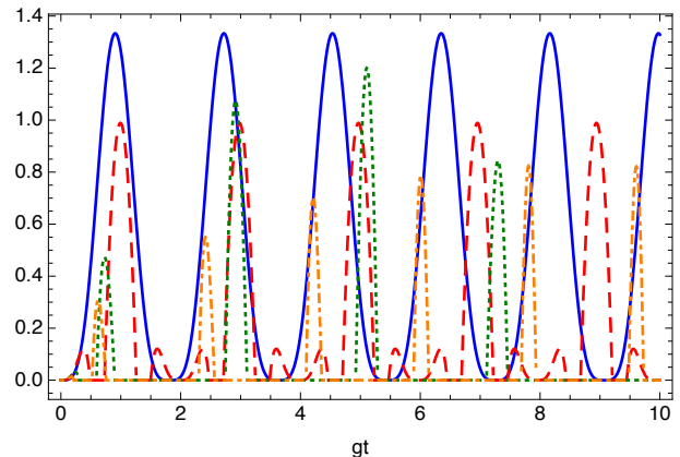
FIG. 3: Entanglement, as indicated by positive values of the left-hand sides of Eqs. (42) and (43), for a system of three atoms starting from the ground state with n_0 = 1 (solid line), 2 (dashed line), 3 (dotted line) and 4 (dot-dashed line) photons respectively. For n_0 = 1 , only the left-hand side of (43) contributes (i.e., is greater than zero). For larger n_0 , however, its contribution is limited to small secondary minima, here only visible for n_0 = 2 .
