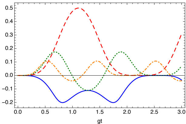
FIG. 2: For the same initial conditions as in Figure 1, the figure shows -\lambda'_4 (where \lambda'_4 is the only eigenvalue of the partial transpose of the matrix (40) that can become negative). The negativity N(\rho) = \max\{0, -\lambda'_4\} ; a positive value of the negativity is a necessary and sufficient condition for entanglement in this system.
