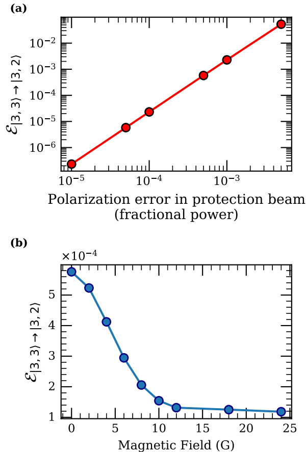
FIG. 8. Scheme 2 polarization error in EIT protection beam. (a) A varying fractional power is applied in the wrong \pi -polarization in the protection beams (with no magnetic field). The main source of error is population transfer |3, 3\rangle \rightarrow |3, 2\rangle through a four-photon Raman transition. (b) Keeping the fractional power at 5 \times 10^{-4} , a magnetic field of varying size is applied in order to reduce the error.
