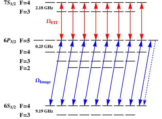
FIG. 2. Scheme 1 EIT-protected detection on the D2 line. The imaging light uses \sigma^+ -polarization and the EIT protection beam uses \pi -polarization. With this configuration all F=4 sublevels are EIT-protected except |4, 4\rangle , which can be imaged on the cycling transition |4, 4\rangle \rightarrow |5', 5'\rangle . For clarity, in this and all similar figures, we do not show the Zeeman shifts of hyperfine levels. EIT protection is quite insensitive to these shifts, as long as they are very small compared to \Omega_{EIT} , which they are in the regime of interest. The wavelength of the imaging light should be chosen to match the imaging transition.
