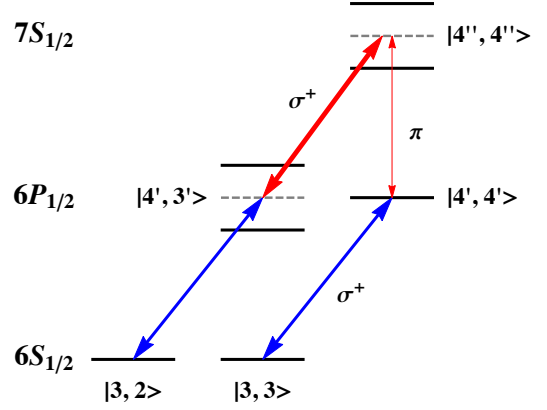
FIG. 7. Scheme 2 possible error caused by a small amount of the wrong \pi -polarization in the protection beam. The \pi -polarization (denoted by the thin red arrow), which would otherwise resonantly couple |4',4'\rangle to a bare |4'',4''\rangle (upper right dashed grey line), is off-resonant due to the strong \sigma^+ (denoted by the thick red arrow), which Rabi-splits |4'',4''\rangle (upper right solid black lines).
