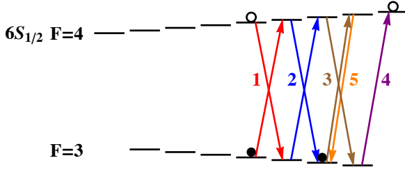
FIG. 9. Selective transfer of an atom out of the qubit basis. The first step (1) in the sequence requires site-specificity, while the remaining steps do not, as they are not resonant with atoms in the qubit states.
