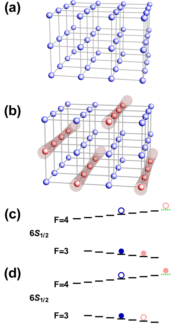
FIG. 1. Overview of the measurement. (a) Initially, atoms in a 3D optical lattice are in random superpositions in the qubit basis (shown in blue). (b) A select group of atoms are transferred to states out of the qubit basis (shown in red, with a red beam going through them). (c) The qubit and non-qubit bases in the Cs ground state. The empty (filled) circle dark blue states are transferred to the empty (filled) circle light red states using a series of stimulated pulses. The red state population in the dotted green sublevel is detected, the other F = 4 states are EIT-protected, and the F = 3 states are protected from light scattering by being far from resonance. (d) Another series of stimulated pulses exchanges the empty and filled circle red states, allowing the other state population to be detected.
