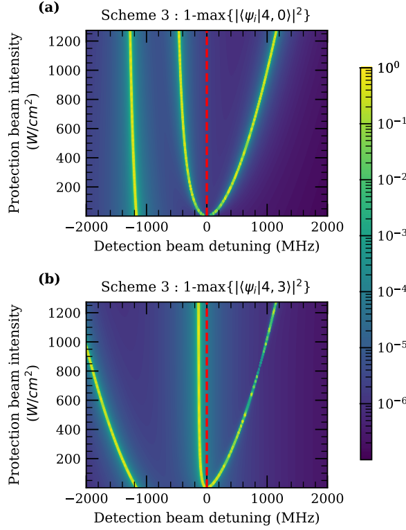
FIG. 16. Scheme 3 dressed states results. The non-ground state population of the nominally EIT-protected states |4,0\rangle (a) and |4,3\rangle (b) as a function of the detection beam detuning and the protection beam intensity. The red dashed line marks where the detection beam is resonant with the cycling transition.
