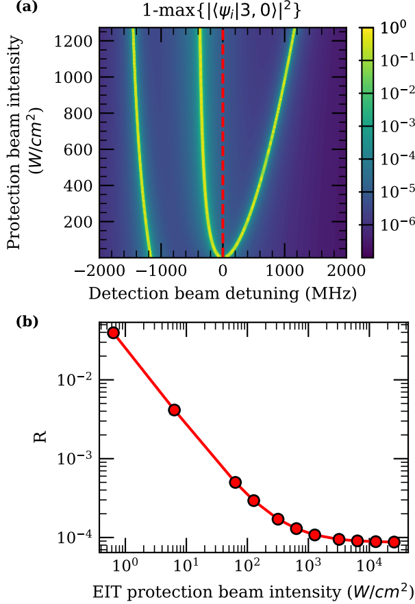
FIG. 6. Scheme 2 results. (a) The non-ground state population of the EIT-protected qubit state |3,0\rangle as a function of the detection beam detuning and the protection beam intensity. The red dashed line marks where the detection beam is resonant with the open transition for imaging. (b) The suppression factor for the reabsorption of scattered photons ( R ) as a function of intensity of the protection beam.
