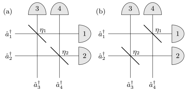
FIG. 2. Discrimination of Bell-like states, with two beam splitters defined by \eta_1 and \eta_2 . As described in Eqs. (34) and (35), in (a) modes 1 and 3 interact in the first beam splitter and modes 2 and 4 interact in the second. In (b), modes 1 and 4 interact in the first beam splitter and modes 2 and 3 interact in the second.
