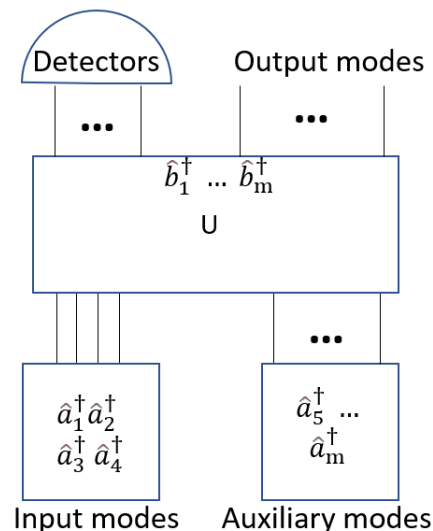
FIG. 1. The general scheme for linear optical operations. The input modes, \hat{a}_i^{\dagger} (the system, i = 1, 2, 3, 4 ) and the auxiliary modes (the ancilla, i = 5, \dots, m ) are coupled via a network of beam splitters and phase shifters to form the output modes. The action of the linear optic network can be described by a total unitary transformation U . At the output, some of the modes are measured using photon resolving detectors, while the remaining undetected modes can be used as input for further processing.
