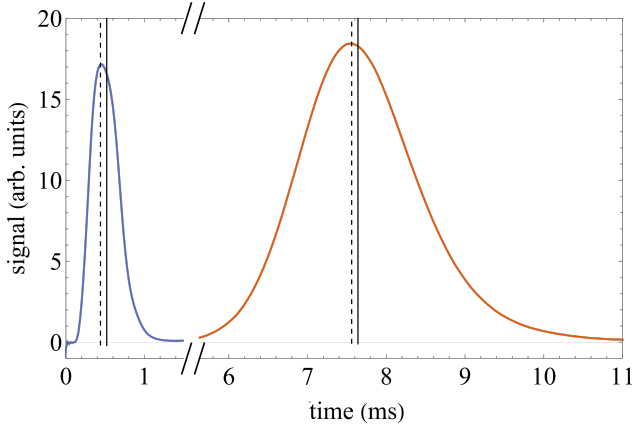
Figure 4. Average absorption near the molecule source (blue, left) and fluorescence in the detection region (orange, right) traces show the transit time and the longitudinal velocity dispersion of the molecular pulses. The peak time (dotted) and average time (solid) differ slightly. The displayed traces are averaged from the entire second data set. The height of the absorption signal has been inverted and re-scaled so it can be compared to the detected fluorescence signal.
