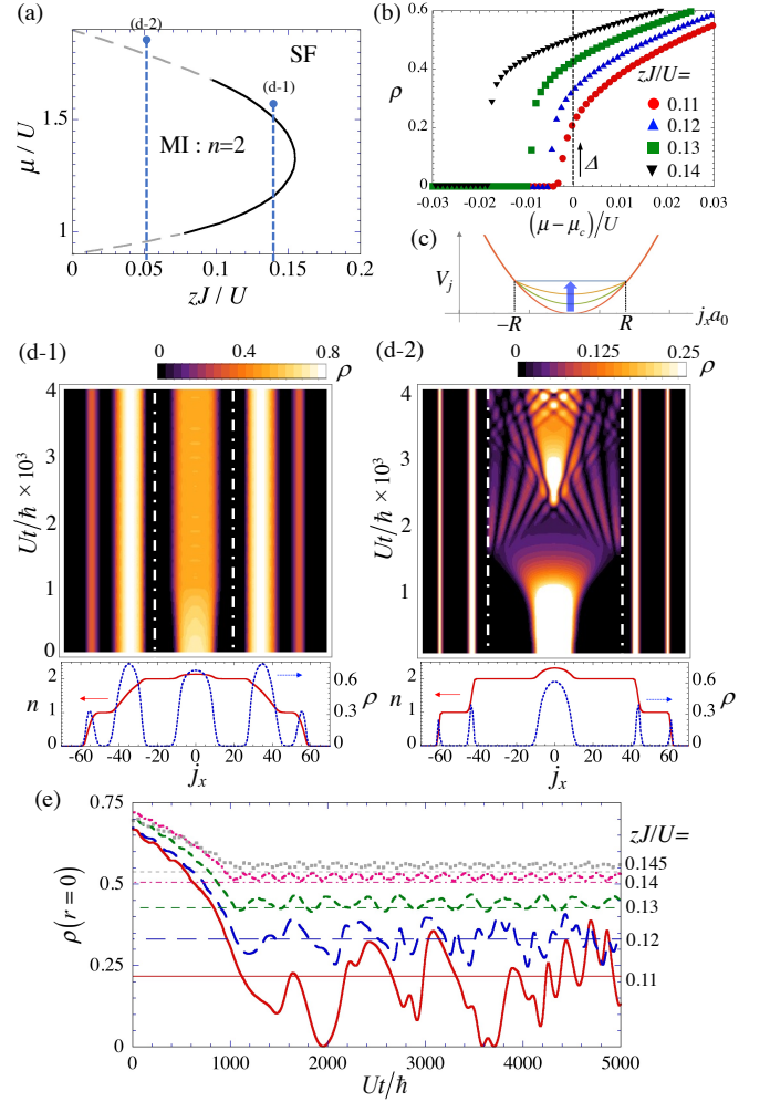
FIG. 1. The panel (a) shows the ground state phase diagram in the zJ/U - \mu/U plane obtained by the Gutzwiller analysis of the BH model Eq. (1) [23, 24]. The solid and dashed curves between SF and MI represent the first and second order transitions, respectively. The vertical dashed lines show the radial dependence of the equilibrium phase in the bottom panels of (d), determined by the local chemical potential. The panel (b) shows the equilibrium condensate density \rho = \sum_{\alpha} |\Psi_{\alpha}|^2 for several values of zJ/U as a function of the chemical potential \mu measured from the transition point \mu_c . For \mu < \mu_c the SF state is metastable. In (c), we show how to change the trap potential for inducing characteristic behavior of a droplet formed by the SF in the central region of the trap. The panels (d) show the time evolution of the cross section of the SF density along the x -axis starting from the initial states of the bottom panels, in which the profiles of the total particle density n_1 + n_2 (red solid curve) and the SF density \rho (blue dashed curve) are shown. The parameters are U_{12}/U = 0.9 , \tilde{k} = 0.001 , and (zJ/U, \mu/U, R) = (0.14, 1.56, 21) for (d-1) and (0.05, 1.85, 35) for (d-2). Here, \mu is chosen as \mu = \mu_c + 0.05U . The vertical dashed-dotted lines show the radius j_x = \pm R of the flat potential area. The panel (e) shows the time evolution of the condensate density at the center for several values of zJ/U . The horizontal thin lines show the gap \Delta of the condensate density at the transition points for the corresponding zJ/U , obtained in (b).
