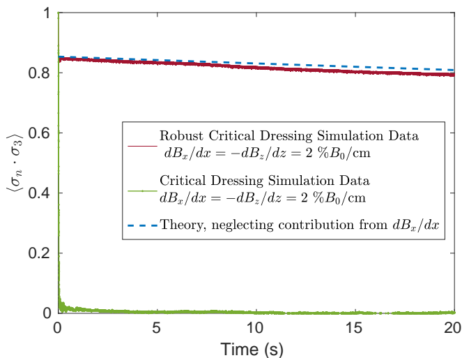
FIG. 9. Simulated signal for highly tuned RCD modulated at 200 \text{ Hz} (red) and CSD (green), with theoretical estimation for RCD (blue). The starting phase for {}^3\text{He} is \phi_3 = \pi/8 , and it is the same for neutrons, \phi_n = \pi/8 . Signal is observable for a long time in the RCD scenario, while the signal is indistinguishable from noise in a traditional critical dressing scenario.
