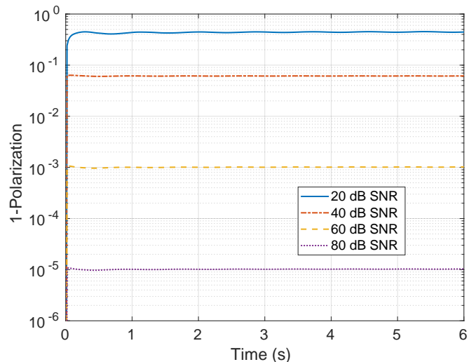
FIG. 8. 1- Polarization for robust dressing modulated according to equation 86, where B_1 = 40.2497 \mu\text{T} and \omega_m = 200 \text{ Hz} , with simulated noise power varied from 20 dB SNR to 80 dB SNR
