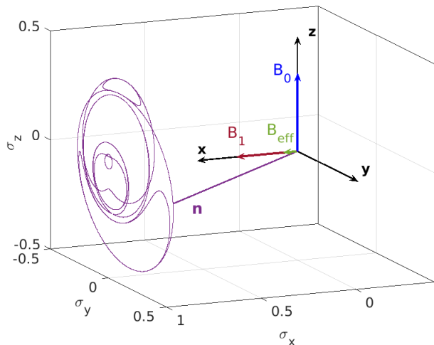
FIG. 6. A classical visualization of the neutron spin trajectory undergoing robust dressing on the Bloch sphere in the laboratory frame, with arrows representing the static uniform field, B_0 , the dressing field, B_1 , and the robust dressing effective field B_{\text{eff}} .
