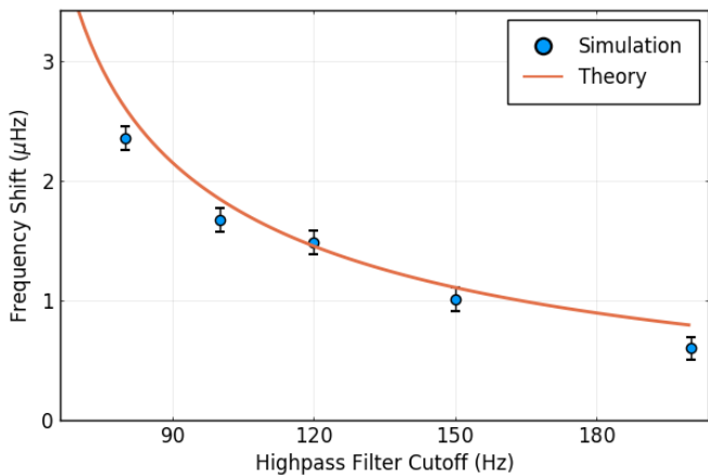
FIG. 3. Predicted and simulated frequency shifts, with magnetic field noise given by equation (83), for various high-pass filter cutoffs. The theory line is calculated from equations (71) and (83). Each simulated point represents 100,000 neutrons.
