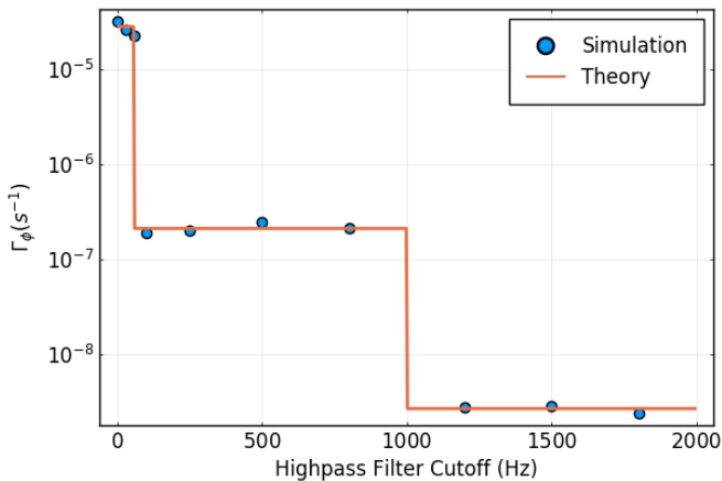
FIG. 2. Predicted and simulated values of \Gamma_\phi for various high-pass filter cutoffs. The theory line is calculated from equations (70) and (83). Each simulated point represents 200 neutrons. Note that cutoff values beyond the dressing frequency (1000 Hz) are only achievable in simulation, and are shown here for comparison to the theory.
