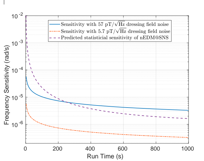
FIG. 1. Run-to-run uncertainty in the measured frequency due to dressing field noise for 57 pT/ \sqrt{\text{Hz}} and 5.7 pT/ \sqrt{\text{Hz}} dressing field noise and a perfect band-pass filter around the dressing frequency, calculated from equation (76). The predicted per-run sensitivity for the nEDM@SNS, formulated from reference [9], is shown for comparison. It is shown that 57 pT/ \sqrt{\text{Hz}} dressing field noise will significantly reduce the ultimate sensitivity of the measured frequency, while 5.7 pT/ \sqrt{\text{Hz}} dressing field noise is acceptable.
