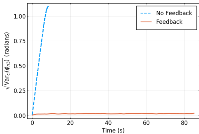
FIG. 4. The root mean squared deviation of the angle between the neutron and ^3\text{He} spins ( \phi_{n3} ) as a function of time, with dressing field powered by a Kepco four-quadrant 400 36-12 power supply, for magnetic fields generated with (solid line) and without (dashed line) feedback control. The dataset without feedback consists of 28 runs, while the dataset with feedback consists of 50. Data are smoothed for clarity.
