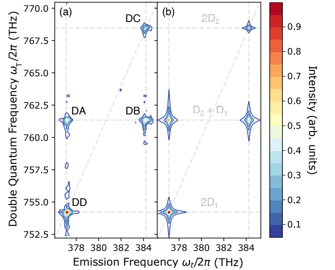
FIG. 7. (a) Experimental and (b) simulated double-quantum 2D spectra of a Rb vapor. The spectral amplitude is plotted with the maximum normalized to 1.
