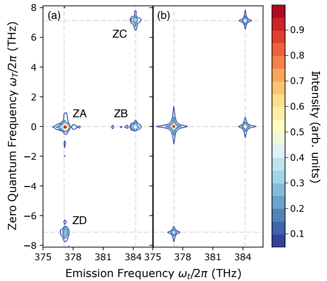
FIG. 5. (a) Experimental and (b) simulated zero-quantum 2D spectra of a Rb vapor. The spectral amplitude is plotted with the maximum normalized to 1.
