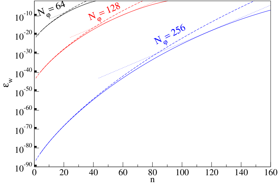
FIG. 3. Tail weight \epsilon_w(n) , Eq. (30), (solid lines) of HG functions versus n for N_\phi = 64 (upper, black), N_\phi = 128 (middle, red) and N_\phi = 256 (lower, blue) discretization points. Eq. (54) (dashed lines) is a good approximation for small n \lesssim 0.3N_\phi . For larger n , \epsilon_w(n) = \epsilon_c(n-2)/(1.5\sqrt{n(n-1)}) with \epsilon_c(n) given by Eq. (61), (dotted lines) provides a better bound for the error.
