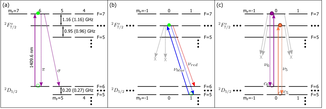
FIG. 4. Ion-photon entanglement protocols discussed in the text, where dotted circles represent the initially prepared atomic state(s), filled circles represent the state(s) excited by the laser pulse, solid lines represent the transition(s) driven by the laser pulse, dotted lines represent decay (photon emission) transitions, and the hyperfine splittings are calculated from the experimental (theoretical) hyperfine A and B coefficients given in Ref. [42] (Ref. [43]). Energy-level diagrams are partial and not to scale. Wavelength given in air [44]. (a) Polarization-encoded photonic qubit: The polarization of the photon (here \pi and \sigma ) is entangled with the final atomic state. Collecting photons in a direction perpendicular to a quantization axis defined by an external magnetic field, \pi and \sigma polarizations are linearly polarized and orthogonal. (b) Frequency-encoded photonic qubit: The (resolved) frequency of the emitted photon (here \nu_{red} and \nu_{blue} ) is entangled with the final atomic state. Collecting photons along a quantization axis defined by an external magnetic field allows filtering-out \pi -polarized light (vertical, gray, dotted line with X) based on the dipole radiation pattern, and \sigma^+ -polarized light (diagonal, gray, dotted line with X) using a quarter-wave plate and polarizer. (c) Amplitude-preserving, frequency-encoded photonic qubit: The (resolved) frequency of the emitted photon (here \nu_5 and \nu_6 ) is entangled with the final atomic state. Collecting photons in a direction perpendicular to a quantization axis defined by an external magnetic field, \pi and \sigma polarizations are linearly polarized and orthogonal, allowing \sigma -polarized light (diagonal, gray, dotted lines with X) to be filtered-out. Conditioned on this filtering, and due to selection rules, the initially prepared atomic amplitudes c_5 and c_6 may be preserved.
