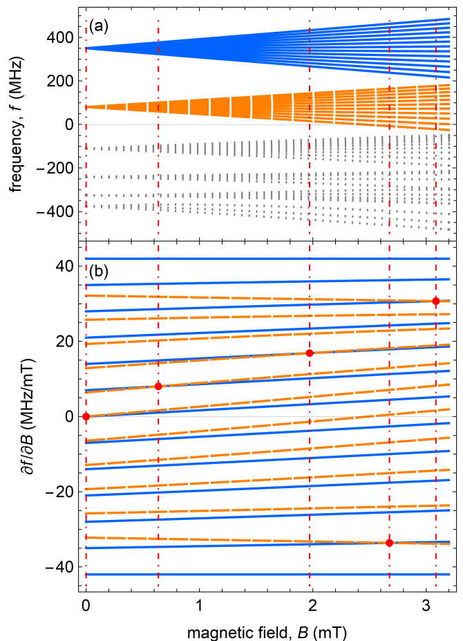
FIG. 2. Calculating the hyperfine interaction in the presence of an external magnetic field is used to identify possible qubit states with splitting first-order insensitive to the magnetic field. (a) Frequency shift ( f ) of states in {}^2D_{5/2} as a function of magnetic field ( B ), using the theoretical hyperfine coefficients from Ref. [43]. (b) First-order derivative of the magnetic field ( \partial f/\partial B ) as a function of the magnetic field ( B ). Solid blue lines are states in the F = 6 manifold, dashed orange lines are states in the F = 5 manifold, red points are where two states have identical derivatives and indicate possible first-order magnetic field insensitive qubits (see Table I), and vertical red dot-dashed lines highlight the strength of the external magnetic field at these points.
