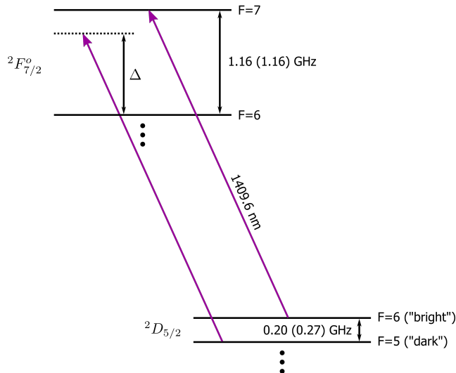
FIG. 3. Qubit state read-out using standard state-dependent fluorescence. Near-resonant, \sigma^- -polarized, laser light drives the {}^2D_{5/2} |F=6\rangle to {}^2F_{7/2} |F=7\rangle transition, driving population in the {}^2D_{5/2} |F=6, m_F=1\rangle qubit state to the cycling transition, scattering many photons and appearing “bright” to a detector. This laser light is detuned from the nearest transition involving the {}^2D_{5/2} |F=5, m_F=1\rangle qubit state by \Delta = 0.96 (0.89) GHz, the difference between the {}^2F_{7/2} F=6 \leftrightarrow 7 and {}^2D_{5/2} F=5 \leftrightarrow 6 hyperfine splittings, and therefore appears “dark” to a detector. Hyperfine splittings are calculated from the experimental (theoretical) hyperfine A and B coefficients given in Ref. [42] (Ref. [43]). Energy-level diagram is partial and not to scale. Wavelength given in air [44].
