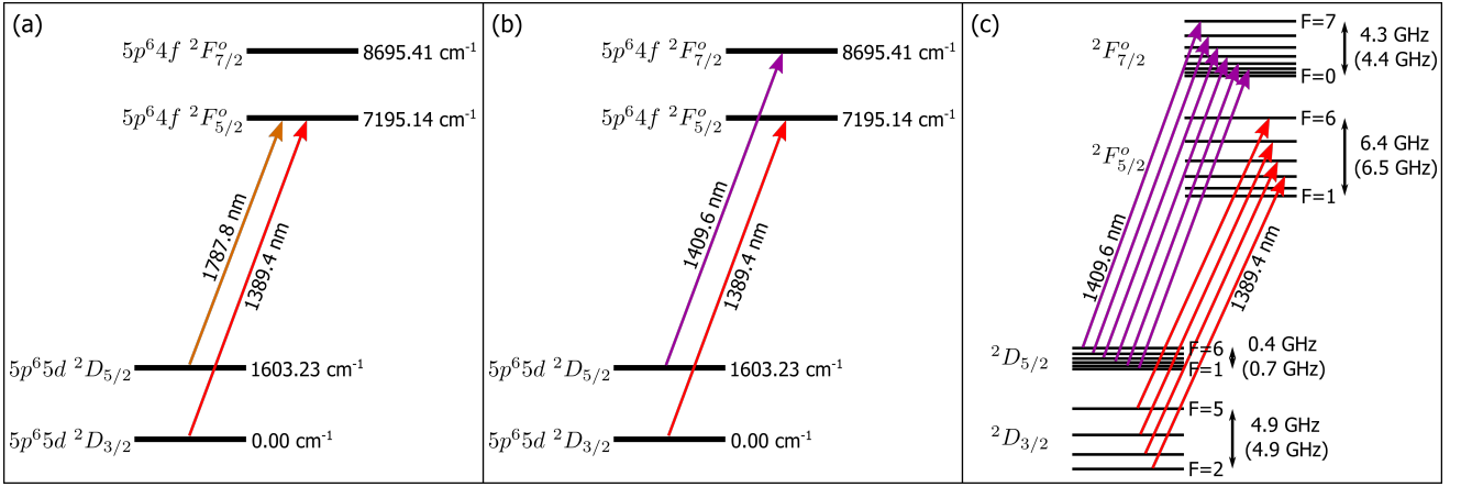
FIG. 1. Energy level diagram of \text{La}^{2+} with possible laser cooling schemes. (a) A 3-level cooling scheme driving the {}^2D_{3/2} \leftrightarrow {}^2F_{5/2}^o transition near 1389.4 nm and the {}^2D_{3/2} \leftrightarrow {}^2F_{7/2}^o transition near 1787.8 nm. (b) A 4-level cooling scheme driving the {}^2D_{3/2} \leftrightarrow {}^2F_{5/2}^o transition near 1389.4 nm and the {}^2D_{5/2} \leftrightarrow {}^2F_{7/2}^o transition near 1409.6 nm. (c) The 4-level cooling scheme with hyperfine structure shown (not to scale), with light driving each {}^2D |F = n\rangle to {}^2F^o |F = n + 1\rangle transition. Here each top (bottom, parenthetical) frequency gives the extent of the hyperfine manifold splitting calculated from the experimental (theoretical) hyperfine A and B coefficients given in Ref. [42] (Ref. [43]). Wavelengths given in air [44].
