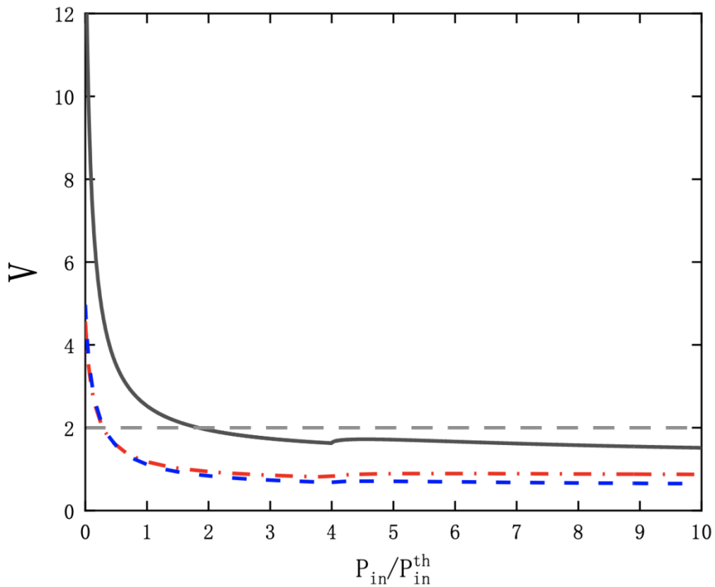
FIG. 3. (Color online) The correlations V_{12} (solid black line), V_{1a} (dot-dashed red line), and V_{2a} (dashed blue line) at zero Fourier frequency as a function of the power P_{1in} = P_{2in} of the two input laser fields, normalized to the threshold power P_{in}^{th} . The other parameters are the same as those in Fig. 2. Below the horizontal gray dashed line the variance is sub-shot-noise. The small features appearing near P_{in} / P_{in}^{th} = 4 are discussed in the text.
