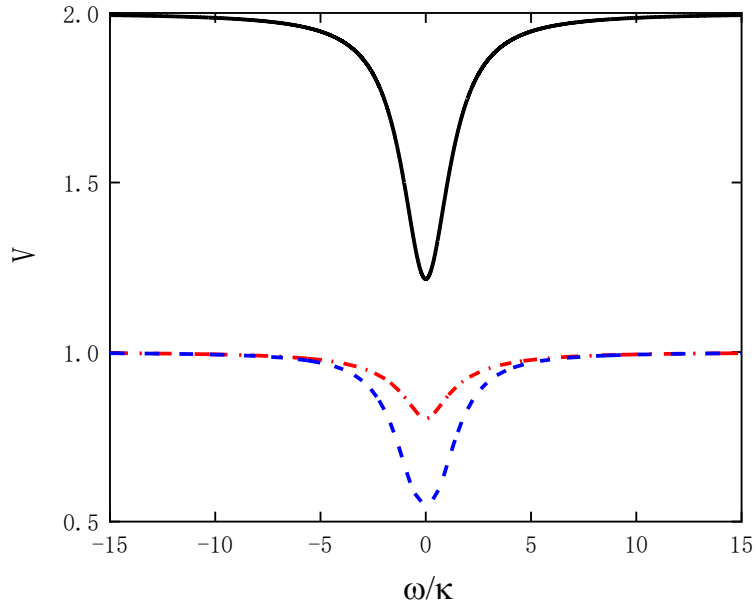
FIG. 2. (Color online) The correlations V_{12} (solid black line), V_{1a} (dot-dashed red line), and V_{2a} (dashed blue line) as a function of the Fourier frequency \omega (normalized to the cavity decay rate \kappa ). V_{12} represents the correlation between the two output cavity fields, and V_{1a, 2a} represents the correlation between the output cavity field 1 (2) and the atoms. The relevant parameters are given in the text.
