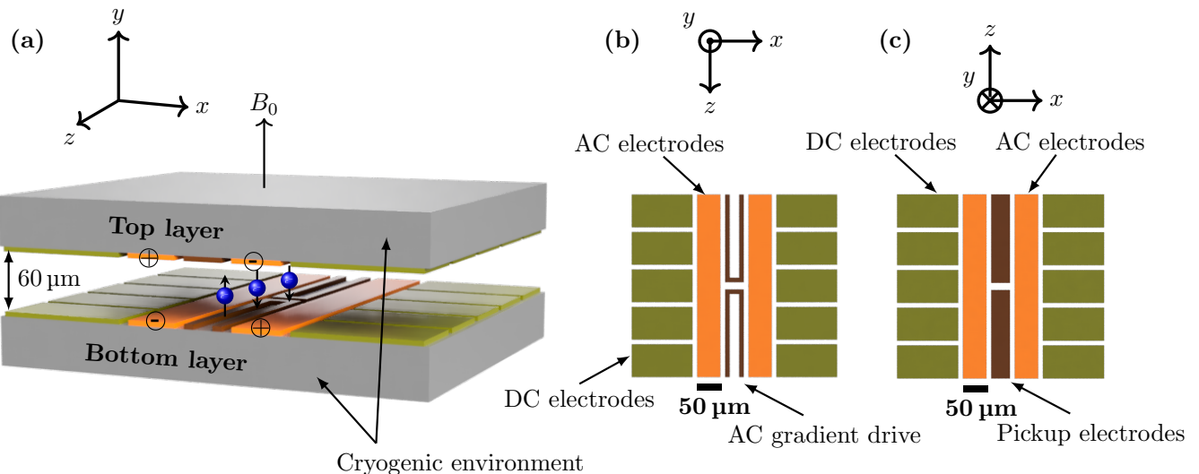
FIG. 1: (a) A prototype trap design provides a framework for analyzing the feasibility of trapped electron quantum computing. The trap consists of two substrates separated by 60\ \mu\text{m} , supporting four AC electrodes that are driven out-of-phase. Driving currents through the two center electrodes of the bottom layer generates a magnetic field gradient or a homogeneous magnetic field (both along the z -axis) depending on the relative phase of the currents. The two center electrodes of the top layer serve to pick up the image current generated by the electron motion. The plus and minus sign at the AC electrodes indicate the phase of the AC drive applied to each electrode. (b) Top view of the bottom substrate. (c) Bottom view of the top substrate.
