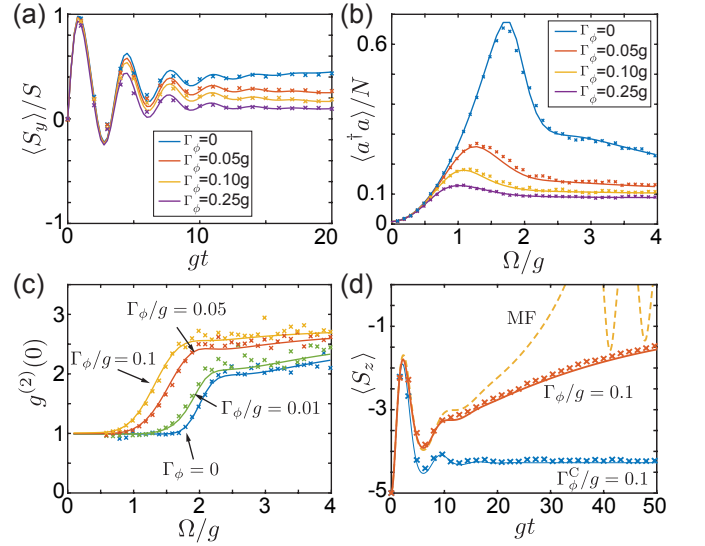
FIG. 6. Simulation of the driven Dicke model as described in Eq. (33) for N = 10 and \kappa = 0.5g , where the spins are initially prepared in the state |\Psi_0\rangle = \prod_i |\downarrow\rangle_i . (a) Time evolution of \langle S_y \rangle for \Omega = 2g and (b) steady state cavity occupation number \langle a^\dagger a \rangle for varying driving strength \Omega . From top to bottom, the different curves in (a) and (b) represent increasing values of the dephasing rate, \Gamma_\phi/g = 0, 0.05, 0.1, 0.25 . (c) Steady state correlation function g^{(2)}(0) as a function of the driving strength \Omega and for different dephasing rates \Gamma_\phi . (d) Evolution of an initial fully polarized spin in the presence of individual ( \Gamma_\phi ) or collective ( \Gamma_\phi^C ) dephasing with the same rate. For this plot \Omega = g . In all the plots the solid lines represent the results obtained from an exact simulation of the master equation exploiting permutational invariance, while the crosses are obtained by the DDTWA method by simulating n_t = 2500 trajectories. In (d) the dashed line shows the prediction from mean-field (MF) theory.
