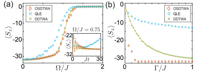
FIG. 8. Comparison of DDTWA with other semiclassical simulation schemes, QLE and OSDTWA, where the magnitude of each classical spin is not conserved on average. (a) Steady state of the transverse Ising model with the same parameters as in Fig. 5. The inset shows that the QLE method does not reach a steady state. (b) Magnetization \langle S_z \rangle at time t = 40/J for a spin model with Hamiltonian H = JS_x^2/N and individual spin decay \Gamma . In both plots N = 64 and the solid lines represent the exact results.
