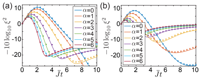
FIG. 4. Time evolution of the squeezing parameter \xi^2 for an ensemble of N = 64 spins arranged on a cubic lattice with unit spacing. The spins are initially aligned along the x -direction, |\Psi_0\rangle = \prod_i |\rightarrow\rangle_i , where |\rightarrow\rangle = (|\uparrow\rangle + |\downarrow\rangle)/\sqrt{2} . For these simulations we assumed \Omega = 0 and individual spontaneous emission of each spin with a rate (a) \Gamma/J = 0.0025 and (b) \Gamma/J = 0.025 . From top to bottom, the different curves represent increasing values of \alpha = 0, 1, \dots, 6 . For a better comparison the curves for different \alpha are plotted in terms of the rescaled time unit \bar{J}^{-1} , where \bar{J} = \sum_{i,j} J_{ij}/N . The solid lines show the exact results [71] for different power-law interactions, as defined in Eq. (27). The crosses show the corresponding values obtained by the DDTWA method for n_t = 10000 trajectories.
