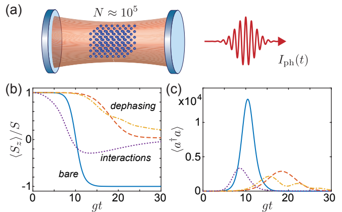
FIG. 7. Superradiant decay of an ensemble of N = 47^3 = 103823 two-level systems that are initially prepared in the excited state and couple to a lossy cavity mode with \kappa = g , as sketched in (a). In (b) we show the decay of the z-magnetization and in (c) the photon number \langle a^\dagger a \rangle \sim I_{\text{ph}}(t) , which is proportional to the emitted field intensity. In both plots we compare the evolution of the bare non-interacting ensemble (blue solid line), with dynamics in the presence of additional Ising interactions \sim \sigma_i^x \sigma_j^x , with J_x/g = 0.025 and \alpha = 3 (purple dotted line). The other two cases show the dynamics of a noninteracting ensemble, but in the presence of local Markovian dephasing with a rate \Gamma_\phi/g = 0.5 (red dashed line) and for an inhomogeneously broadened ensemble (yellow dashed-dotted line). In the latter case the spin frequencies \omega_i have been randomly drawn from a normal distribution with zero mean and a variance of \sigma^2 = 2\Gamma_\phi^2 . To obtain this data, n_t = 64 trajectories were simulated.
