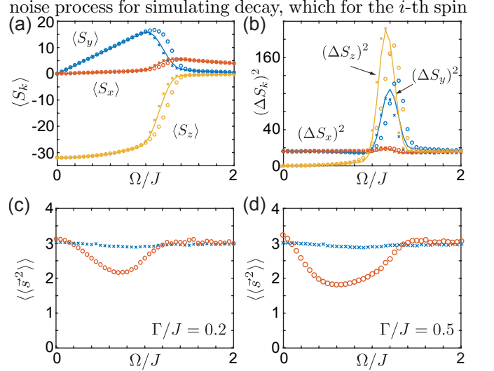
FIG. 9. (a) and (b) The same plots as in Fig. 5 (a) and (b), but for a larger value of \Gamma/J = 0.5 . (c) and (d) Variation of the corresponding average spin length in steady state, \langle \langle \bar{s}^2 \rangle \rangle = \sum_i \langle \bar{s}_i^2 \rangle / N , for two different values of \Gamma . In all plots the solid lines represent the exact results and the circles mark the DDTWA simulations based on the stochastic updates given in Eqs. (21)-(23). The crosses indicate the results obtained via the improved noise process defined in Eqs. (C1)-(C3). All other parameters are the same as in Fig. 5.
