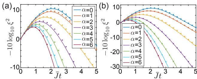
FIG. 2. Time evolution of the squeezing parameter, \xi^2 , for an ensemble of N = 64 spins arranged on a 3D cubic lattice with unit spacing. The spins are initially aligned along the x -direction, |\Psi_0\rangle = \prod_i |\rightarrow\rangle_i , where |\rightarrow\rangle = (|\uparrow\rangle + |\downarrow\rangle)/\sqrt{2} . For these simulations we assumed \Omega = 0 and an individual dephasing of each spin with a rate (a) \Gamma_\phi/J = 0.0025 and (b) \Gamma_\phi/J = 0.025 . From top to bottom, the different curves represent increasing values of \alpha = 0, 1, \dots, 6 . For a better comparison the curves for different \alpha are plotted in terms of the rescaled time unit \bar{J}^{-1} , where \bar{J} = \sum_{i,j} J_{ij}/N . The solid lines show the exact results [71] for different power-law interactions, as defined in Eq. (27). The crosses show the corresponding values obtained with the DDTWA for n_t = 10000 trajectories.
