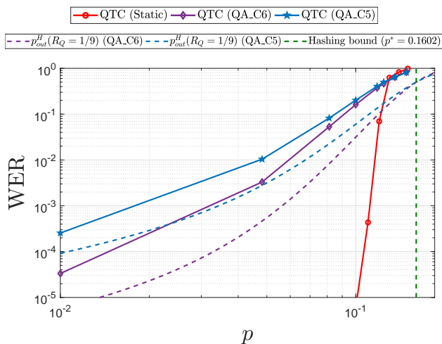
FIG. 4: Performance of the quantum turbo code from [16, 26]. The quantum turbo code operates over the static ADCTA channel and the TVADCTA channel for scenarios QA_C5 and QA_C6 [19, 26]. The quantum error correction code has rate R_Q = 1/9 and encodes blocks of 1000 logical qubits into 9000 physical qubits. The hashing bound and the hashing outage probabilities are also plotted.
