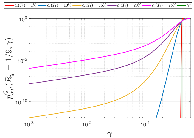
FIG. 1: Quantum outage probability of the TVAD channel. The metric is calculated for TVADs with c_v(T_1) = \{1, 10, 15, 20, 25\}\% and for a quantum rate of R_Q = 1/9 .
