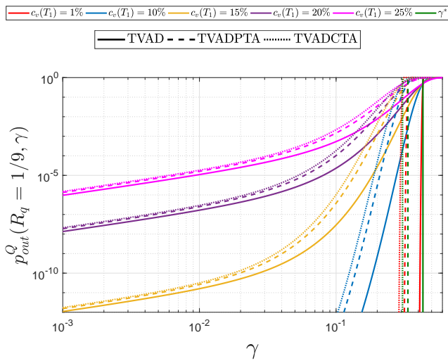
FIG. 3: Quantum outage and hashing outage probabilities for TVAD, TVADPTA and TVADCTA when R_Q = 1/9 . The noise limits are: \gamma_{AD}^* = 0.432 , \gamma_{ADPTA}^* = 0.3354 and \gamma_{ADCTA}^* = 0.3065 .
