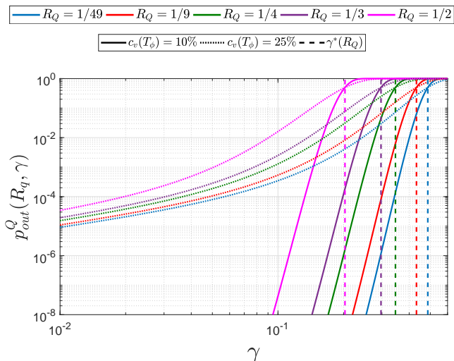
FIG. 2: Quantum outage probability of the TVAD channel for different quantum rates. The considered quantum rates are R_Q \in \{1/49, 1/9, 1/4, 1/3, 1/2\} . We plot the quantum outage probability for c_v(T_1) = \{10, 25\}\% . The quantum capacities (noise limits, \gamma^* ) for the static quantum channels are also represented.
