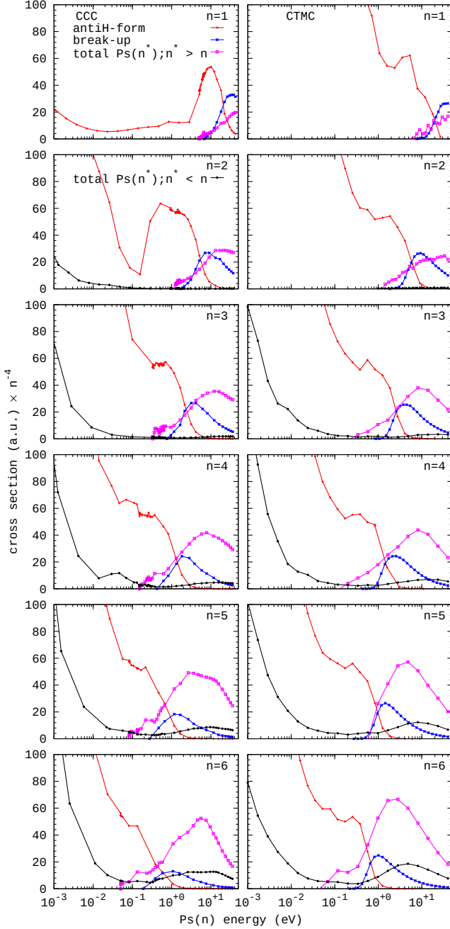
FIG. 2. Integrated cross sections, scaled by n^{-4} , for break-up (reaction 2) and Ps state-changing (reaction 3) for both endo- ( n^* > n ) and exothermic ( n^* < n ) cases (see text) compared to the values for \bar{\text{H}} formation of Fig. 1.
