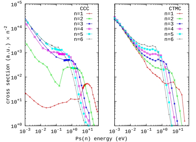
FIG. 1. Total antihydrogen formation cross sections for \bar{p}-\text{Ps}(n) scattering, scaled by n^{-2} (see text). The CCC data are shown in the left panel, with those for the CTMC approach on the right.
