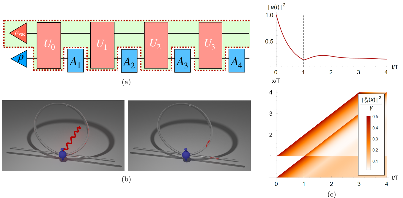
FIG. 1: (a): Scheme of a quantum stochastic process for a system coupled with an environment, initially prepared in a global state \rho_0 = \rho \otimes \rho_{\text{vac}} . At times t_1, \dots, t_4 , an intervention is performed on the system alone; between consecutive interventions, system and environment evolve freely. (b): Scheme of a qubit in a photon waveguide with a two-point interaction. The loop of length T creates a time-delayed coherent feedback and non-Markovian effects on the qubit evolution. (c): Free evolution of |0, \text{vac}\rangle : plot of the survival probability of the emitter |a(t)|^2 (top) and density plot of the wavefunction of the emitted boson |\xi_t(x)|^2 (bottom) for the model with double point interaction, with \gamma T = \omega_0 T = 2 ; darker shades correspond to larger values of |\xi_t(x)|^2 . In both graphs, the dashed black line represents the time t = T at which |a(t)|^2 ceases to be exponential and Eq. (10) ceases to hold. Plotted quantities are dimensionless.
