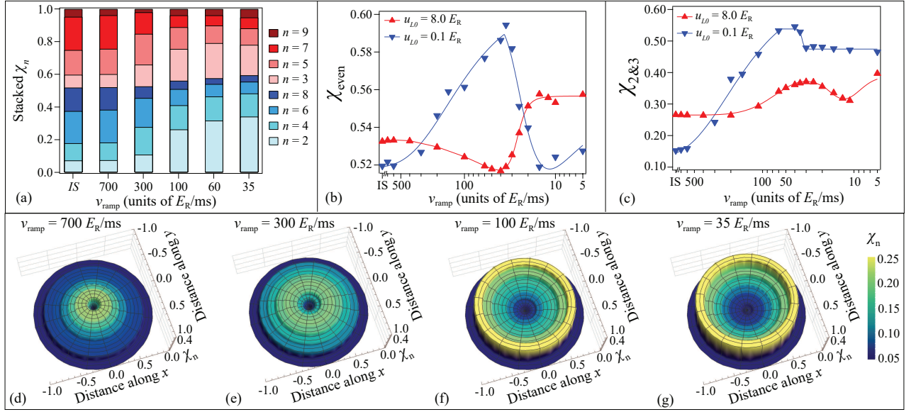
FIG. 4. (a) Predicted number distributions \chi_n derived from our numerical simulations for 2D lattice-confined sodium spinor gases after ramp sequences with u_{L0} = 0.1 E_R at various v_{\text{ramp}} and for IS , the initial superfluid ground state. Shades of blue (red) represent even (odd) n with the shades getting darker as n increases from 2 to 8 (3 to 9). The height of each shaded box represents the predicted \chi_n for a given n , while the combined height of the blue (red) boxes represents the total number distributions in even (odd) Mott lobes. (b) Markers represent fractions of even Mott lobes extracted from simulated lattice quenches similar to those shown in Panel (a) but at various v_{\text{ramp}} and two u_{L0} . (c) Similar to Panel (b) but markers represent \chi_{2\&3} . Solid lines in Panels (b)(c) are fitting curves to guide the eye. (d-g) Similar to Figs. 3(a) - 3(c) but after the simulated quenches at v_{\text{ramp}} = 700, 300, 100 and 35 E_R/\text{ms} respectively.
