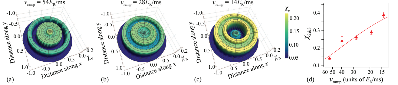
FIG. 3. (a-c) Spatial distributions of atoms corresponding to the measured \chi_n shown in Fig. 2(a) at v_{\text{ramp}} = 54(1) , 28(1) , and 14(1)E_R/\text{ms} , respectively (see text). The z axis and color scale correspond to the observed \chi_n while the radial distance from the center denotes the predicted radii of each Mott plateau and is normalized so that the outer radius of the n = 1 Mott lobe is 1. (d) Markers represent the observed \chi_{2\&3} from the distributions presented in Fig. 2(a). The solid line is an exponential fit.
