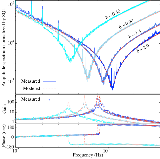
FIG. 3. Demonstration of the dip-shaped spectrum from the amplitude fluctuation of the input light. The amplitude spectrum normalized by the SQL is shown at the upper panel, and the openloop transfer function is shown at the middle and bottom panels. The experiment is performed in four different detunings, and the results (blue solid curves and points) are fitted by the modeled curves (red dotted lines). The estimated normalized detunings ( \delta \equiv \Delta/\kappa ) are written along the measured spectra.
