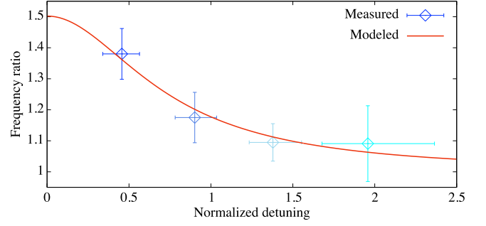
FIG. 4. Ratios between optical spring frequencies and dip frequencies. The four blue dots with errors represent the results with the different detunings. Each colored dot corresponds to the estimation from the same colored spectrum in Fig. 3. The red line shows the modeled curve fitted to the measured data.
