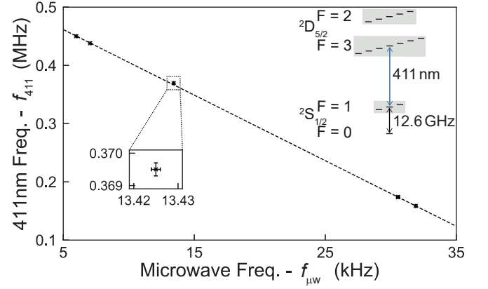
FIG. 4. Frequency of ^2D_{5/2} |F=3, m_F=0\rangle near 411 nm vs. frequency of ^2S_{1/2} |F=1, m_F=0\rangle with respect to ^2S_{1/2} |F=0\rangle at different magnetic field strengths. They are deduced from the ^2S_{1/2} |F=1, m_F=1\rangle \leftrightarrow ^2D_{5/2} |F=3, m_F=0\rangle and the ^2S_{1/2} |F=0\rangle \leftrightarrow ^2S_{1/2} |F=1, m_F=0\rangle transitions which are illustrated on the right. Typical statistical uncertainties of the frequency measurements are approximately 200 Hz and 0.2 Hz for the optical and microwave frequencies, respectively, with the error bar size highlighted in the lower inset. The frequency offsets used for plotting are f_{\mu w} = 12.642812118466 \text{ GHz} , and f_{411} = 729.487559 \text{ THz} . We deduce a slope of -11.27(4) where the uncertainty is the standard error of the fit.
