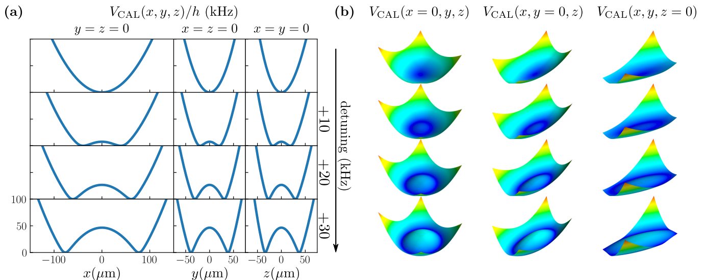
FIG. 8. (Color online) Spatial slices (a) and qualitative surface plots (b) of the CAL trap at various detuning frequencies. In contrast to the bubble trap, the CAL trap is anisotropic, hence the images are shown along different spatial axes. Each consecutive row of images corresponds to a higher detuning frequency, with the first row corresponding to the initial or “bare” trap.
