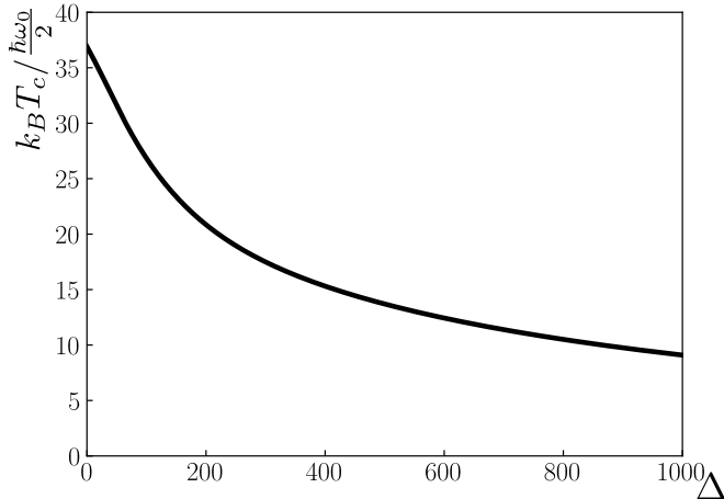
FIG. 3. The BEC critical temperature of N = 5 \times 10^4 bosons in the bubble trap versus the detuning parameter \Delta , which controls the shell thickness. \Delta = 0 \rightarrow 1000 corresponds to continuously deforming the system from a filled-sphere to hollow thin-shell (Fig. 1). The temperature is given in units of \frac{\hbar\omega_0}{2k_B} where \omega_0 is the oscillator frequency in Eq. (2).
