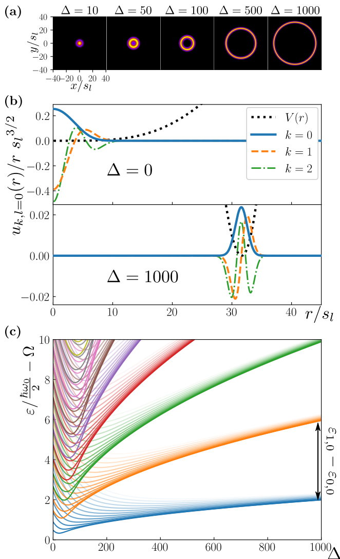
FIG. 2. (Color online) Eigenstates and spectrum of the noninteracting bubble-trapped system (a) Probability density for the ground state wavefunction in the z = 0 plane at various detuning values. In each plot, the color is normalized such that black (yellow) corresponds to the minimum (maximum) value. (b) Radial components of wavefunctions in the bubble trap, u_{k,l=0}(r)/r . Only the zero angular momentum states for k = 0, 1, 2 are shown (along with a shifted and scaled potential in the background). We show the wavefunctions in the two extreme limits of a filled-sphere, \Delta = 0 , and a thin-shell, \Delta = 1000 . (c) Partial spectrum of the bubble trap with the potential minimum, \Omega \frac{\hbar\omega_0}{2} , subtracted off. The color is based on the index k , with k = 0 corresponding to blue, k = 1 corresponding to orange, and so on. As l increases, so does the corresponding energy level \varepsilon_{kl} for a given k . Higher angular momentum states have been removed from the image for clarity.
