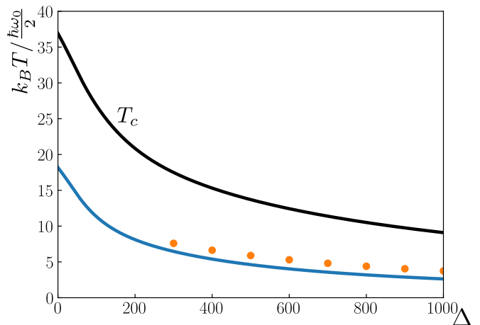
FIG. 7. (Color online) Bubble trap expansions of N = 5 \times 10^4 atoms done at a fixed-condensate fraction N_0/N . The black line shows the noninteracting (NI) BEC critical temperature, whereas the colored lines show the temperature required for an 80% condensate fraction. The solid lines correspond to NI data whereas the markers correspond to Bogoliubov collective excitations. Because this Bogoliubov formalism assumes the NI condensate wavefunction is a reasonable approximation to the GP equation, we only show data points for \Delta \geq 300 where this assumption can be justified.
