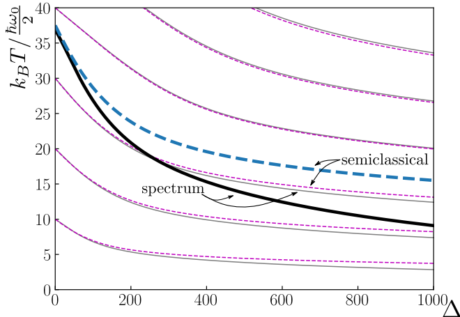
FIG. 5. (Color online) Comparison of our previous results using the spectrum of the bubble trap with the semiclassical approximation. Here, we show the BEC critical temperature for N = 5 \times 10^4 particles along with various adiabatic expansion temperature profiles. [The undashed (dashed) black (blue) line is T_c using the spectral (semiclassical) approach. The undashed (dashed) grey (magenta) lines are adiabatic expansion profiles using the spectral (semiclassical) approach.]
