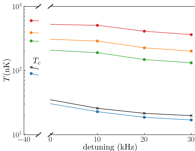
FIG. 9. (Color online) BEC critical temperature (black line) of N = 5 \times 10^4 noninteracting ^{87}\text{Rb} atoms in the CAL trap along with various adiabatic expansion temperature profiles (colored lines) calculated semiclassically. The adiabatic expansions use experimentally-relevant initial temperatures in [32]: T_i = 90, 290, 390, 600 nK.
