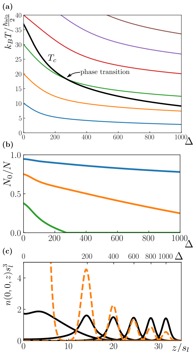
FIG. 4. (Color online) (a) BEC critical temperature (black line) of N = 5 \times 10^4 particles in the bubble trap along with various adiabatic expansion temperature profiles (colored lines). Each adiabatic expansion corresponds to a different initial temperature when \Delta = 0 : k_B T_i / \frac{\hbar\omega_0}{2} = 10, 20, 30, \dots . Note that T_c decreases faster than any adiabatic temperature profile; thus, expanding the gas isentropically leads to a decreasing condensate fraction. (b) Plot of the condensate fraction, N_0/N , during the adiabatic expansions shown in the previous image. (c) Comparison of the local condensate density (colored-dashed lines) and excited state density (black-solid lines) at various stages of the k_B T_i = 20 \frac{\hbar\omega_0}{2} adiabatic expansion (shown along the z -axis). Above each density curve is the associated value of \Delta (marked at the potential minimum location s_l\sqrt{\Delta} ).
