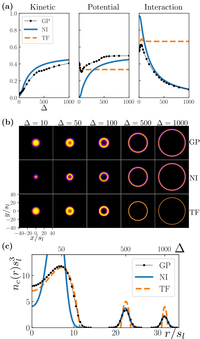
FIG. 6. (Color online) Comparison between the zero-temperature Gross-Pitaevskii (GP), noninteracting (NI), and Thomas-Fermi (TF) condensate wavefunctions at various detunings for N = 5 \times 10^4 atoms in the bubble trap. (a) From left to right, the fraction of energy stored as kinetic, trap potential, and interaction energy. Note: the bubble trap reference energy has been subtracted off from the potential. We also treated quantum depletion as nearly negligible for the NI condensate wavefunction [38] (we set N_0 = 0.99N for T = 0 ). (b) Local condensate density at various detunings. The density is plotted in the z = 0 plane: n_c(x, y, 0) = |\psi_c(x, y, 0)|^2 . In each plot, the color is normalized such that black (yellow) corresponds to the minimum (maximum) density value. (c) Local condensate density plotted against the radial coordinate for the detunings \Delta = 50, 500, 1000 displayed in (b).
