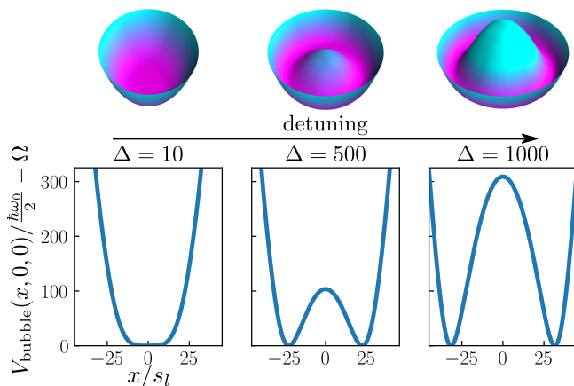
FIG. 1. (Color online) Top (bottom) row: surface plots (spatial slices) of the bubble trap at various detuning values. As \Delta increases, the location of the radially symmetric potential minimum, s_l\sqrt{\Delta} , expands outwards leading to the formation of shell-shaped structures.
